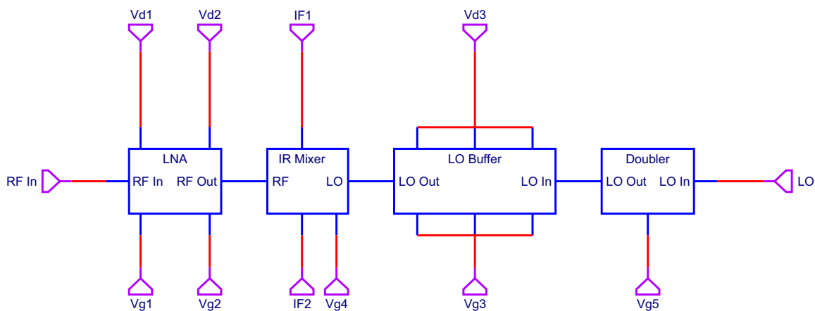
Block Diagram
