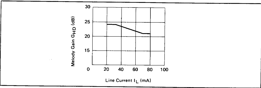
MELODY GAIN VS. LINE CURRENT
