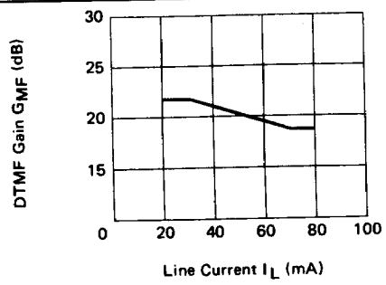
DTMF GAIN VS. LINE CURRENT
