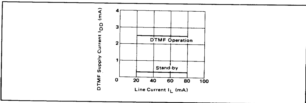
DTMF SUPPLY CURRENT VS. LINE CURRENT
