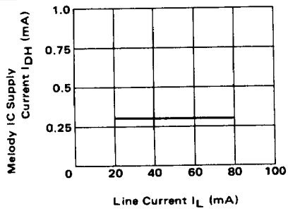
MELODY IC SUPPLY CURRENT VS. LINE CURRENT
