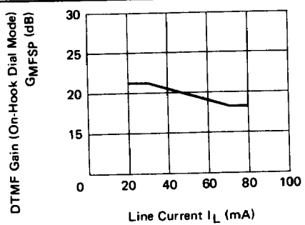
DTMF GAIN (ON-HOOK DIAL MODE) VS. LINE CURRENT
