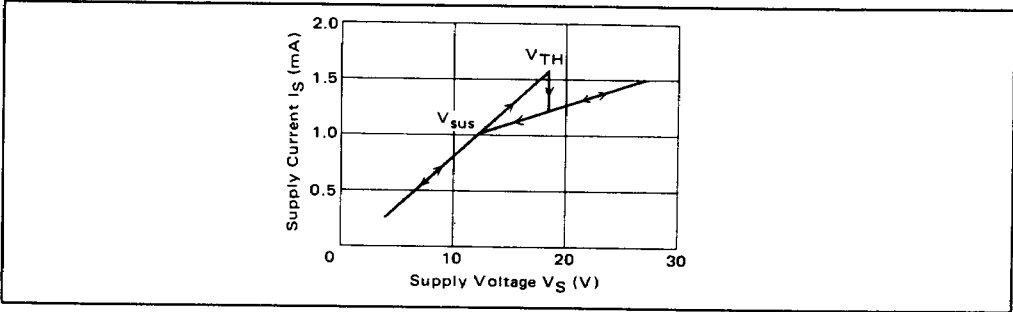
TONE RINGER SUPPLY VOLTAGE VS. SUPPLY CURRENT
