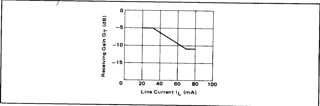
RECEIVING GAIN VS. LINE CURRENT
