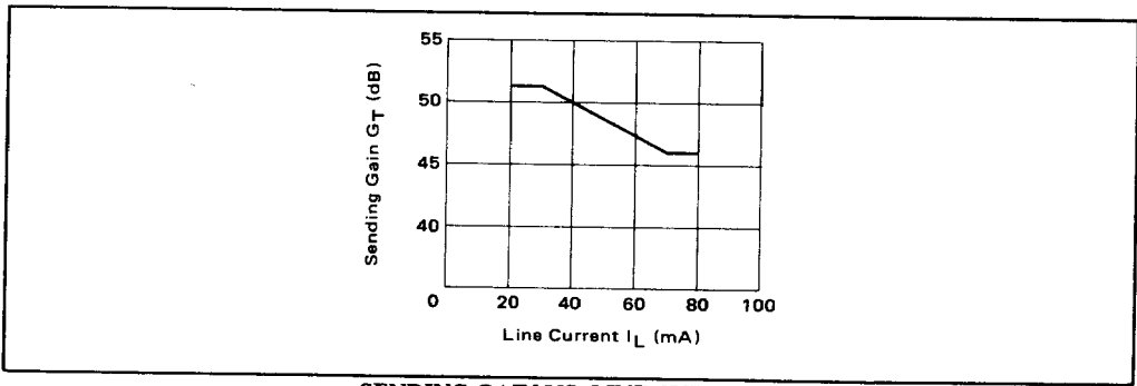
SENDING GAIN VS. LINE CURRENT
