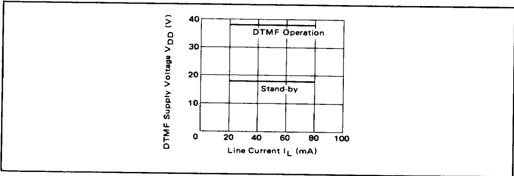
DTMF SUPPLY VOLTAGE VS. LINE CURRENT
