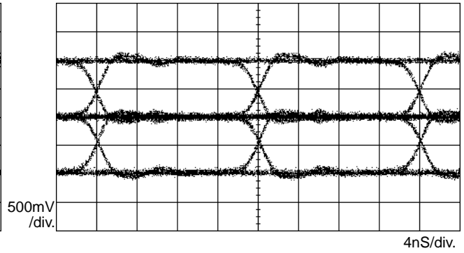
Fig.6 Transmit output MLT-3 data
