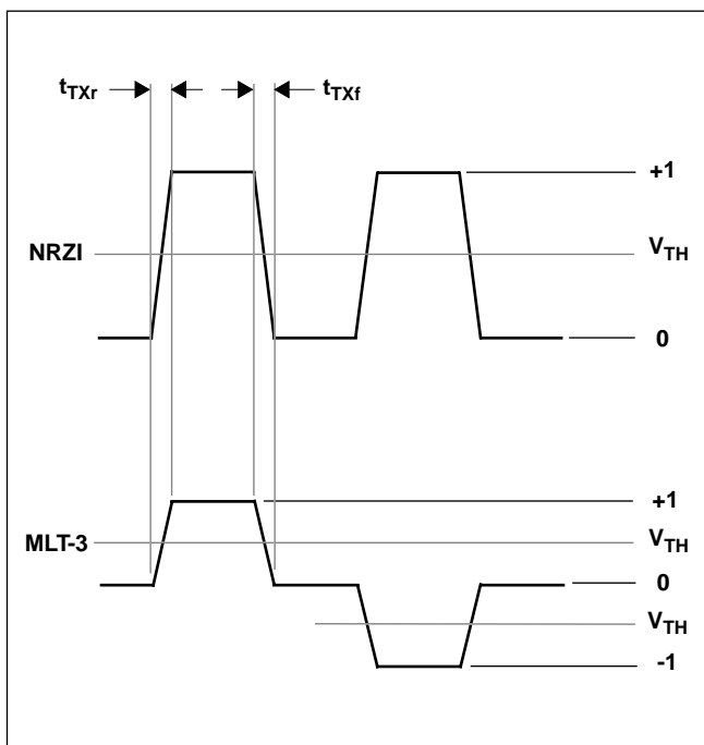
Fig.3 Normalized signal waveforms NRZI/MLT-3
