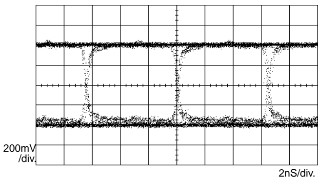
Fig.7 PECL RX data output NRZI mode
