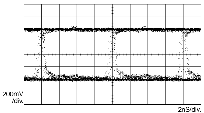
Fig.8 PECL RX data output MLT-3 mode
