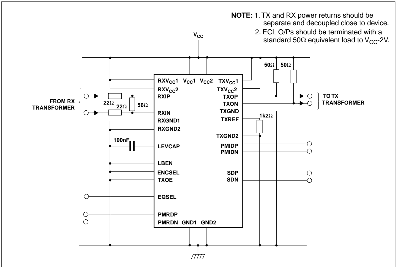
Fig.4 Typical application diagram (MLT-3 100Ω CAT-5 UTP)
