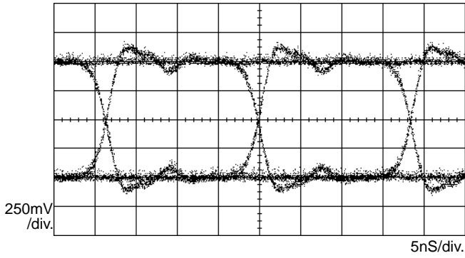
Fig.5 Transmit output NRZI data
