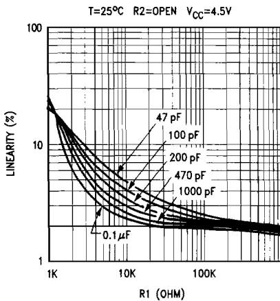
VCO WITHOUT OFFSET R2 = \infty
