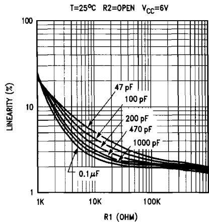
HC4046 Typical VCO Linearity vs R1 & C1
