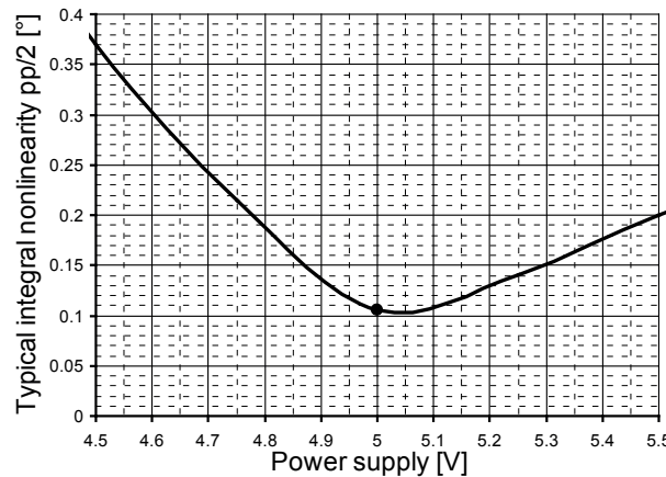
Fig. 28: Accuracy Vs Power supply
