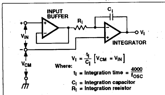
Figure 6 Common-Mode Voltage Reduces Available Integrator Swing ( V_{CM} = V_{IN} )
