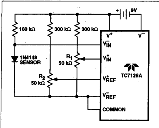
Figure 12 Temperature Sensor
