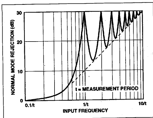
Figure 2 Normal-Mode Rejection of Dual-Slope Converter
