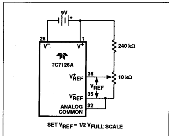
Figure 8 TC7126A Internal Voltage Reference Connection
