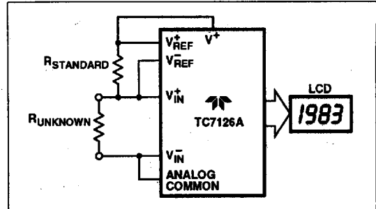
Figure 10 Low Parts Count Ratioetric Resistance Measurement
