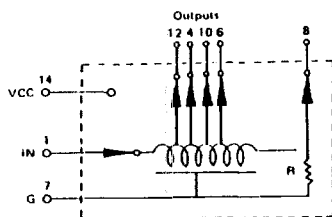
Schematic Diagram For 5 Delays Output
