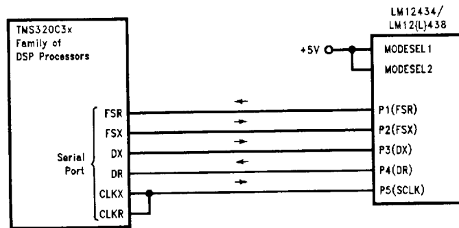
FIGURE 16. LM12434 and LM12(L)438 in the TMS320 Interface Mode
