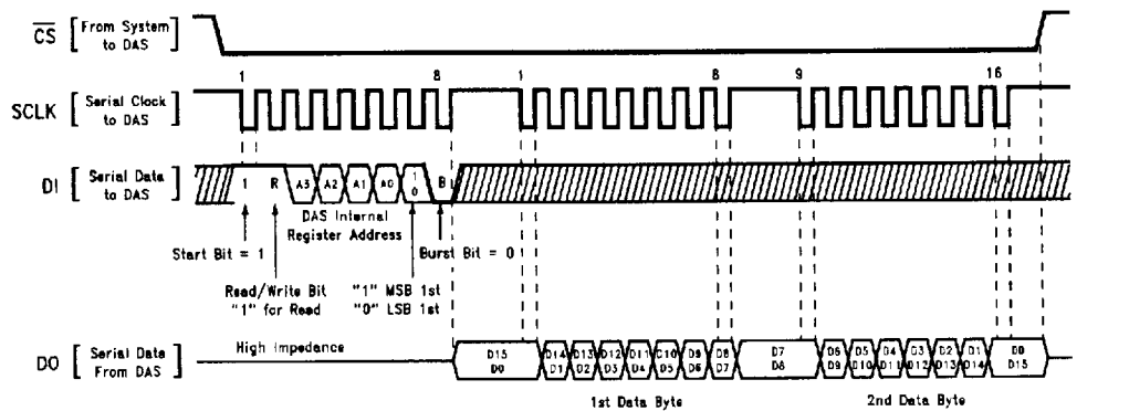
FIGURE 11. Timing Diagrams for LM12434 and LM12(L)438 Standard Serial Interface (Continued)
