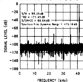
Unipolar Spectral Response with 41.2 kHz Sine Wave at 0 dB Reading Data between Conversions
