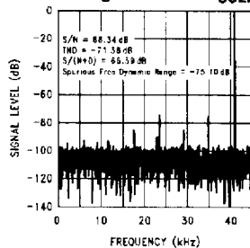
Unipolar Spectral Response with 41.2 kHz Sine Wave at 0 dB Reading Data during Conversion f_{SCLK} = 10\text{ MHz}
