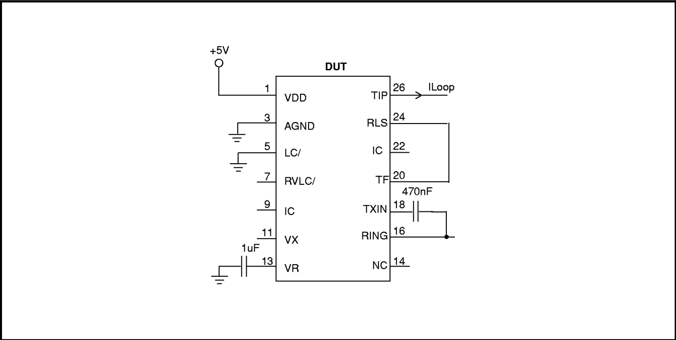
Figure 4 - Test Circuit 1
