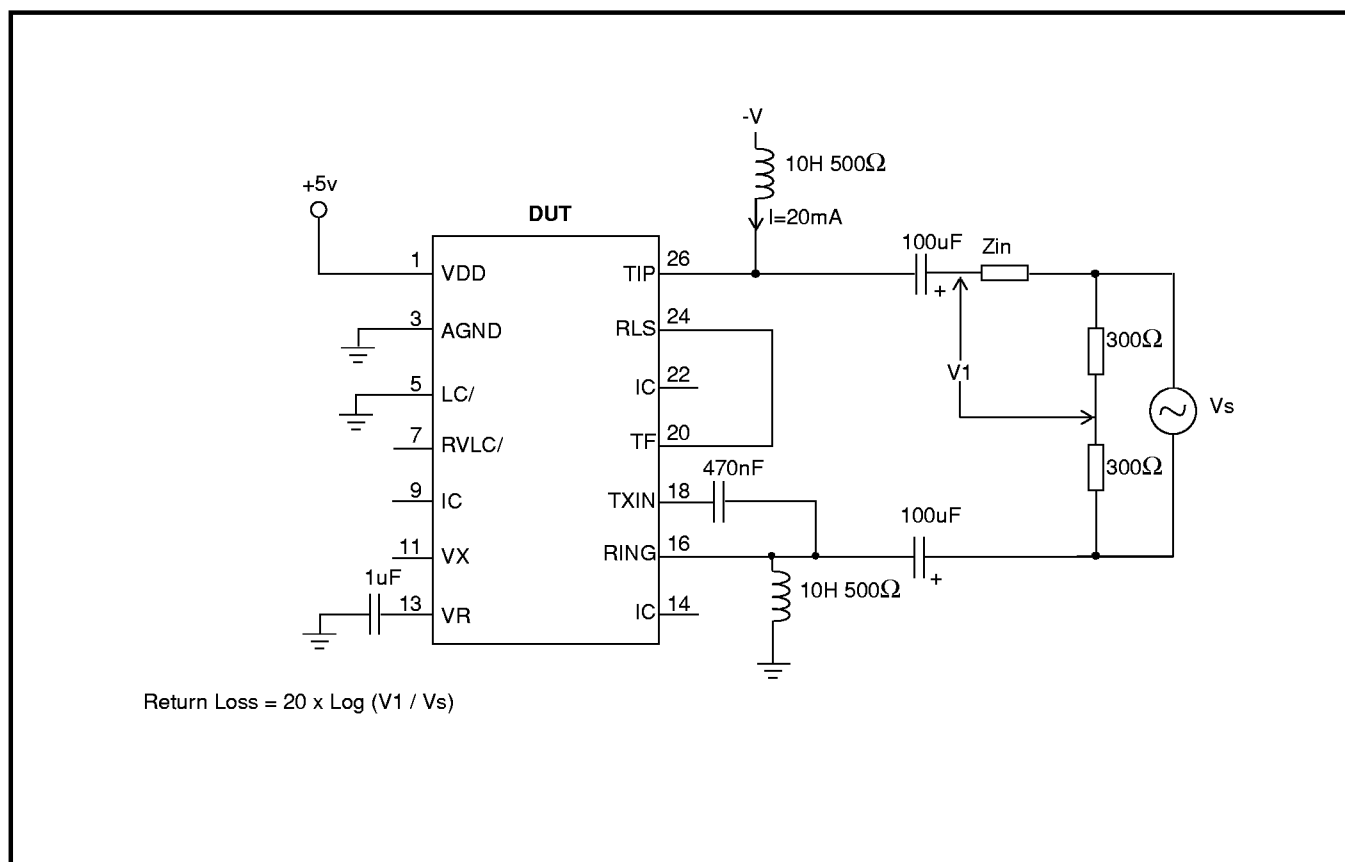
Figure 7 - Test Circuit 4
