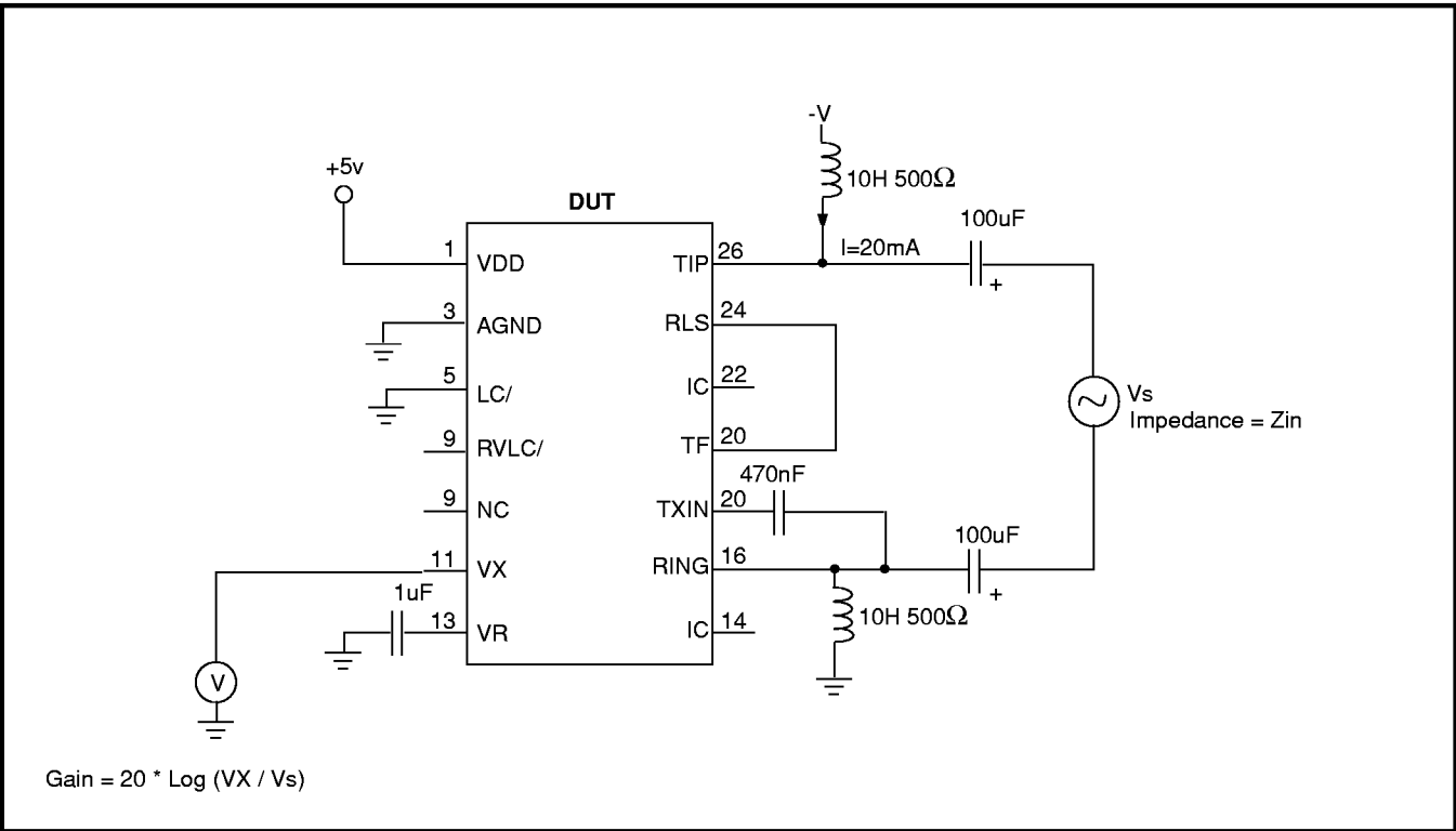
Figure 5 - Test Circuit 2
