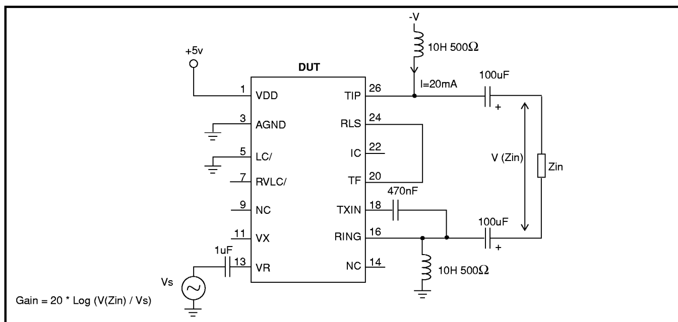
Figure 6 - Test Circuit 3
