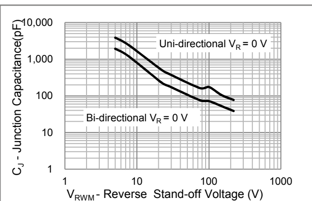
Fig.4 Typical Capacitance
