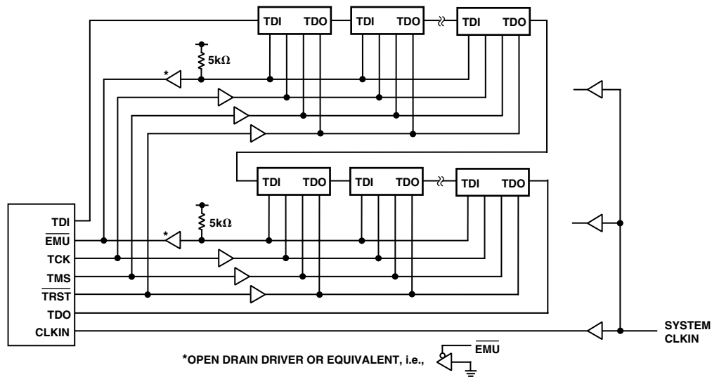
Figure 7. JTAG Clocktree for Multiple ADSP-21061/ADSP-21061L Systems
