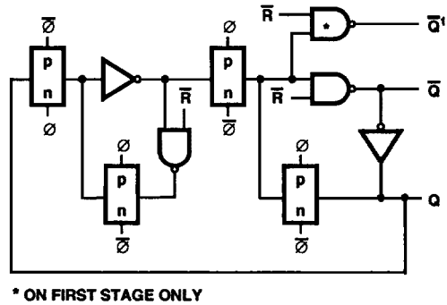
FIGURE 11. DETAIL OF TYPICAL FLIP-FLOP STAGES
