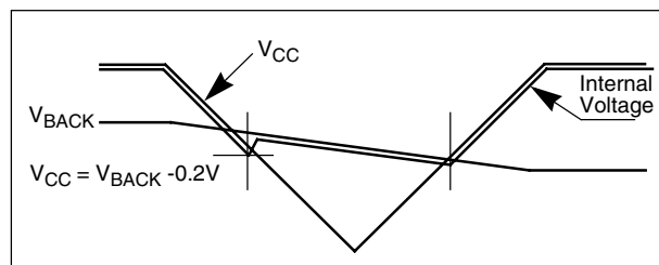
Figure 2. Power Control
