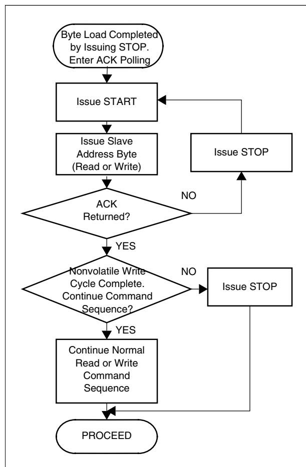
Figure 17. Acknowledge Polling Sequence
