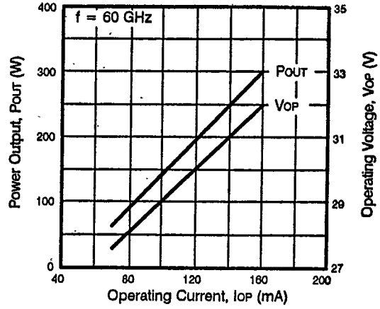
ND8L60W-1T OPERATING CHARACTERISTICS
