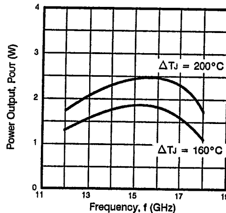
ND8S15W-1N, ND8S15W-5H POWER OUTPUT vs. FREQUENCY
