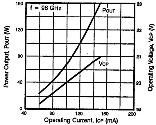
ND8G96W-1T OPERATING CHARACTERISTICS
