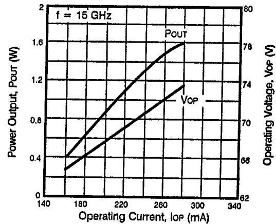
ND8P15-5H OPERATING CHARACTERISTICS
