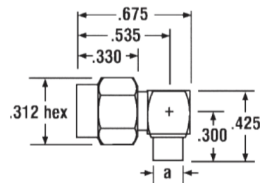
3221-5-9 SMA Right Angle Male Semi-Rigid/Ultra-Flex-Solder RG401 .250 (Passivated)
