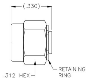
3136-1 SMA Straight Male Semi-Rigid/Ultra-Flex-Solder .034 SR (Gold)
