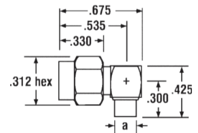
3221-2A-1 SMA Right Angle Male Semi-Rigid/Ultra-Flex-Solder RG405 .085 (Gold)
