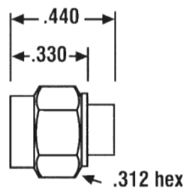
3207-1-1 SMA Straight Male Semi-Rigid/Ultra-Flex-Solder RG402 .141 SR (Gold)
