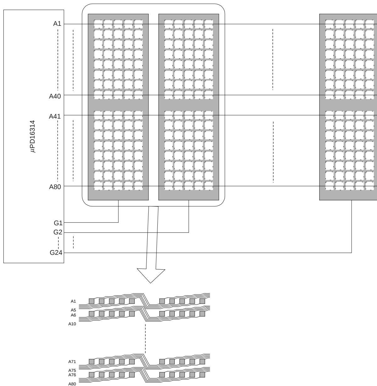
Figure 6-1. VFD Display
