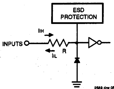
Figure 2. Input Structure
