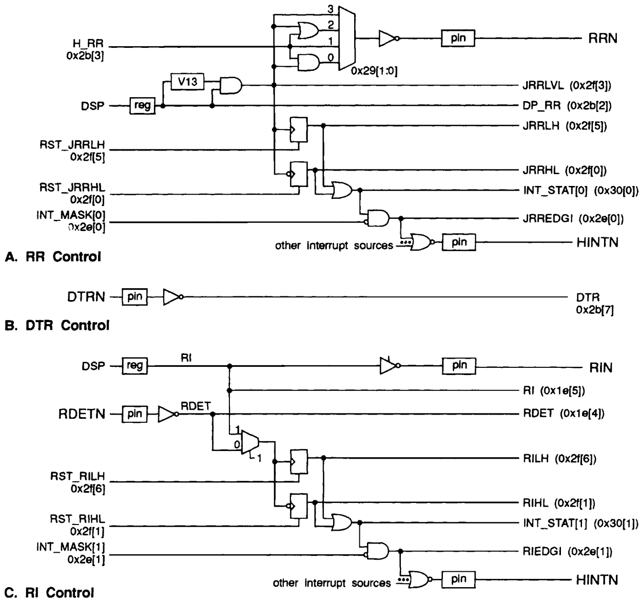
Figure MC-4. V.24 Control Signal Logic
