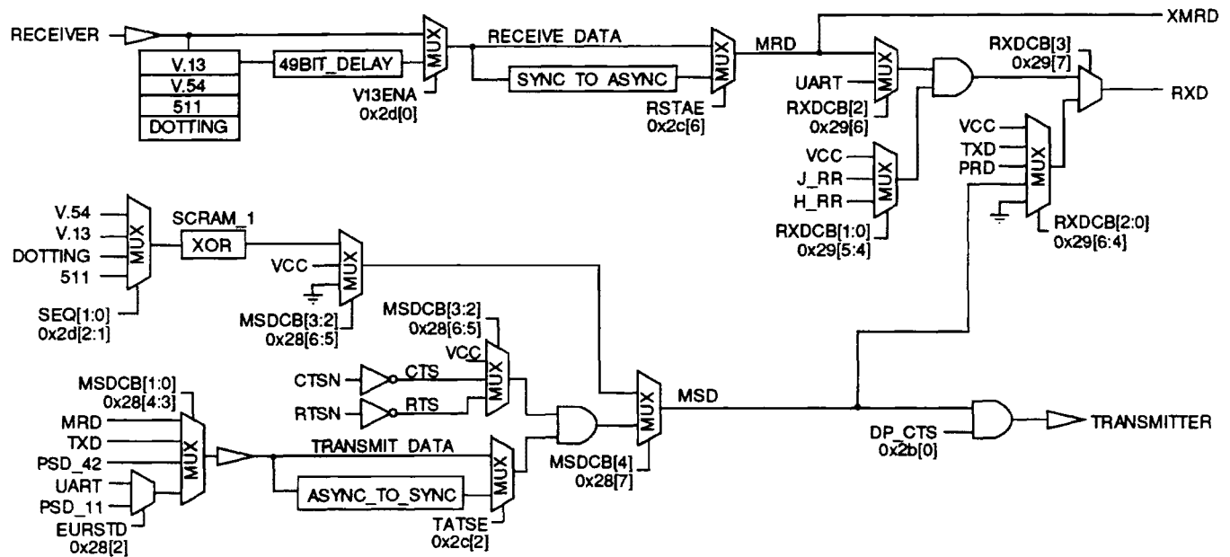
Figure MC-6. EIA Data Path Control
