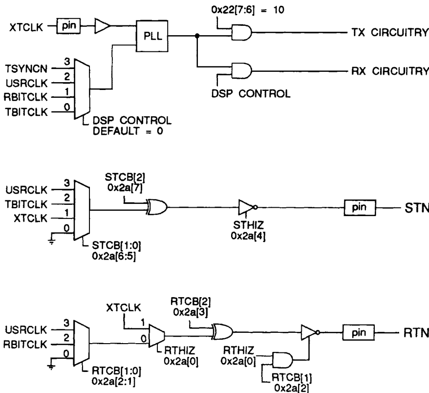
Figure MC-5. V.24 Timing Control
