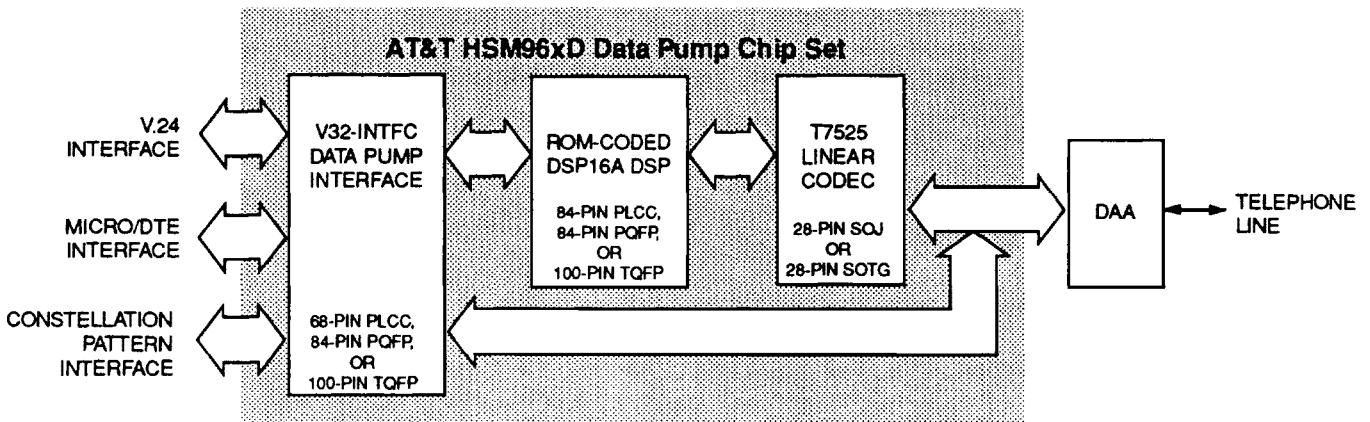
Figure MC-2. Block Diagram of the HSM144xD-V Data Pump
