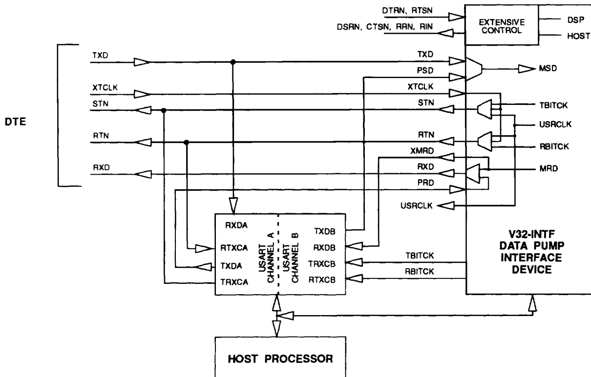
Figure MC-7. V.42 Data and Timing Configuration
