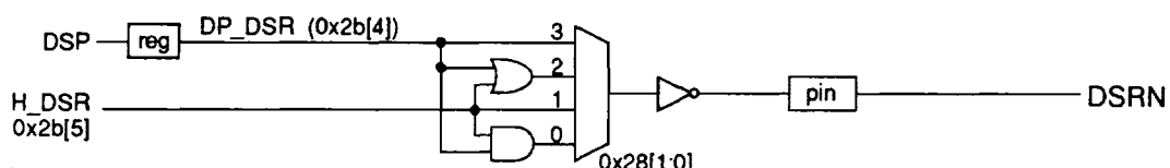
Figure MC-4. V.24 Control Signal Logic (continued)
