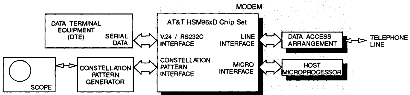
Figure MC-1. Block Diagram of a Modem Using the AT&T HSM96xD Chip Set
