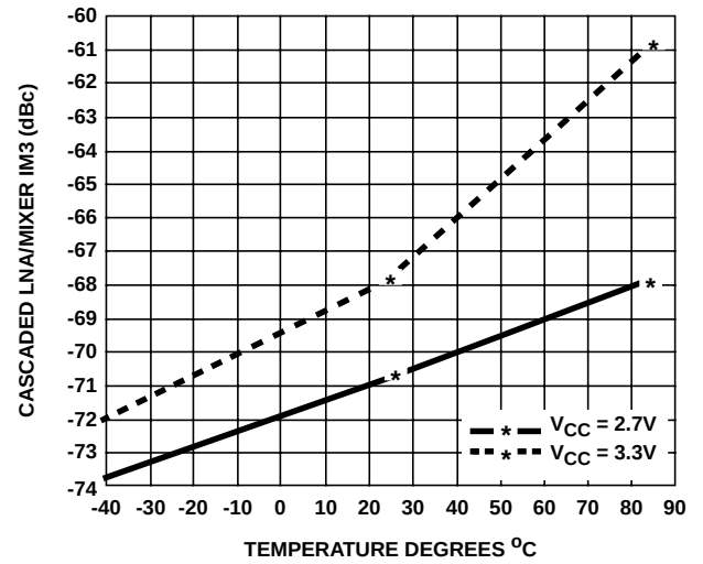
FIGURE 33. RX OUTPUT IM3 AT -20dBm INPUT TONES
