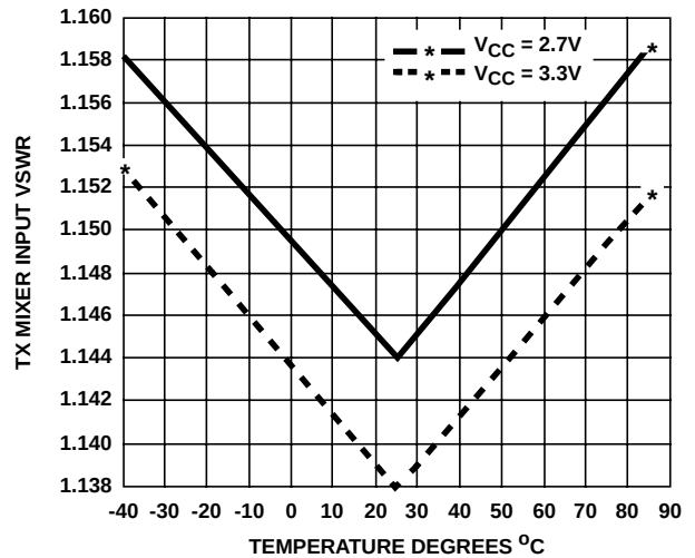
FIGURE 43. TX MIXER INPUT VSWR
