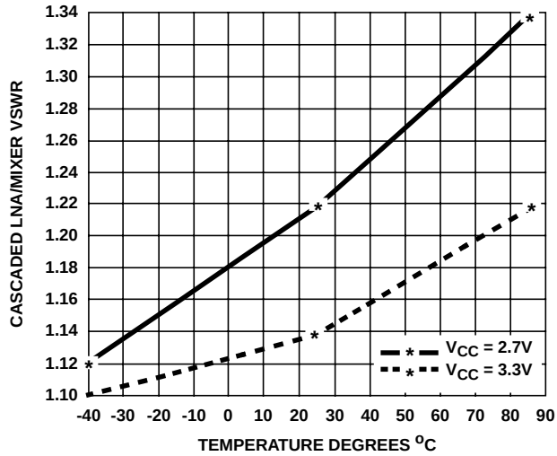
FIGURE 36. LNA INPUT 50Ω VSWR LOW GAIN MODE
