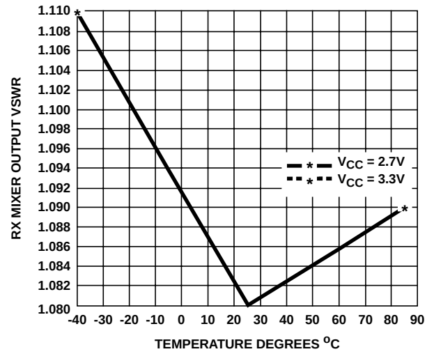
FIGURE 37. RX MIXER OUT VSWR
