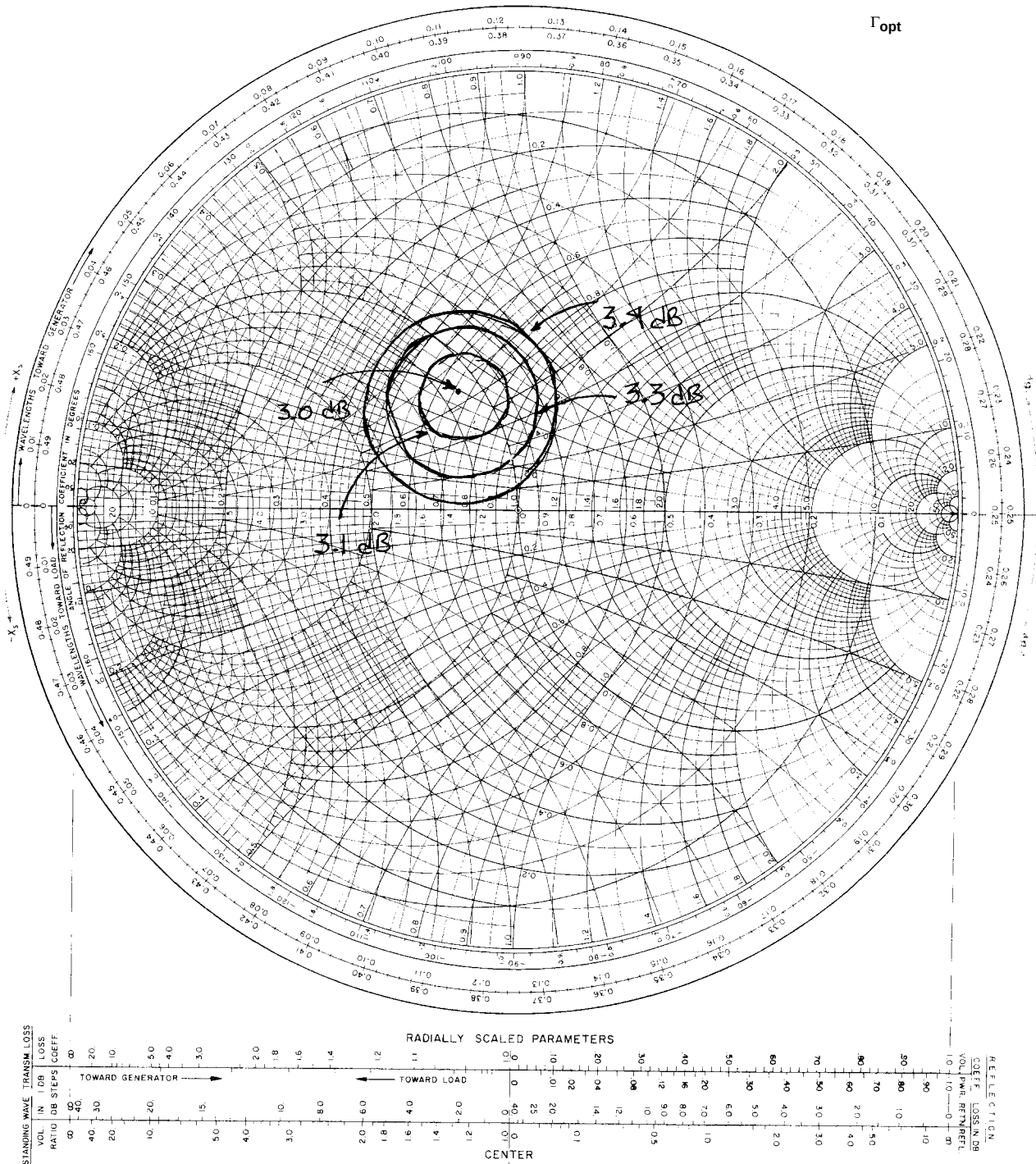
FIGURE 46. GAMMA OPT
