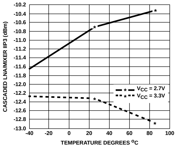
FIGURE 28. INPUT IP3 HIGH GAIN MODE
