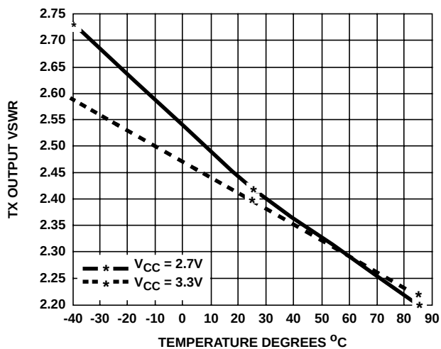
FIGURE 44. PREAMPLIFIER OUTPUT 50Ω VSWR
