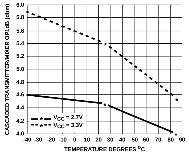
FIGURE 41. OUTPUT P1dB
