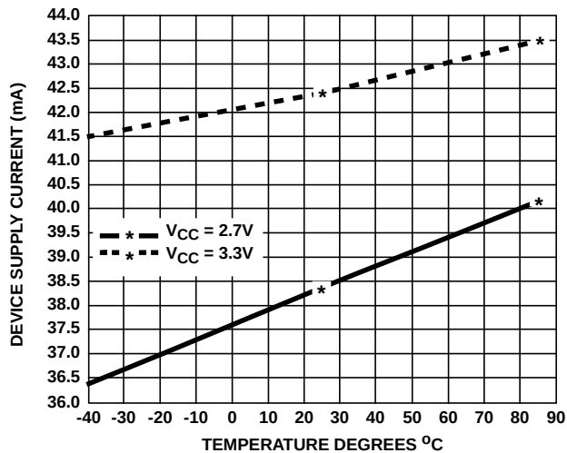
FIGURE 26. TRANSMIT TOTAL SUPPLY CURRENT
