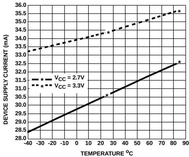
FIGURE 24. RECEIVE TOTAL SUPPLY CURRENT (LNA IN HIGH GAIN)
