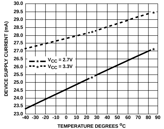
FIGURE 25. RECEIVE TOTAL SUPPLY CURRENT (LNA IN LOW GAIN)
