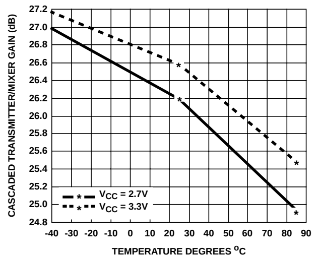
FIGURE 39. POWER CONVERSION GAIN
