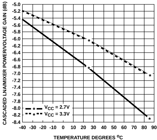
FIGURE 30. POWER/VOLTAGE GAIN LOW GAIN MODE
