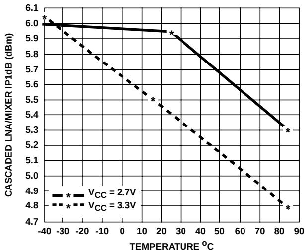
FIGURE 34. INPUT P1dB LOW GAIN MODE
