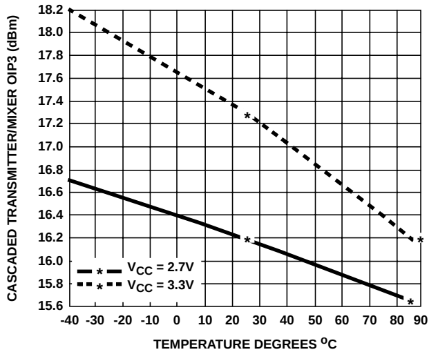
FIGURE 40. OUTPUT IP3
