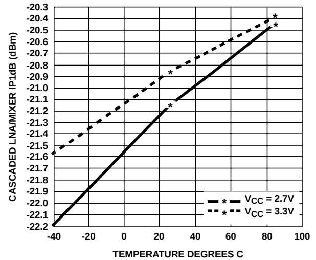
FIGURE 29. INPUT P1dB HIGH GAIN MODE
