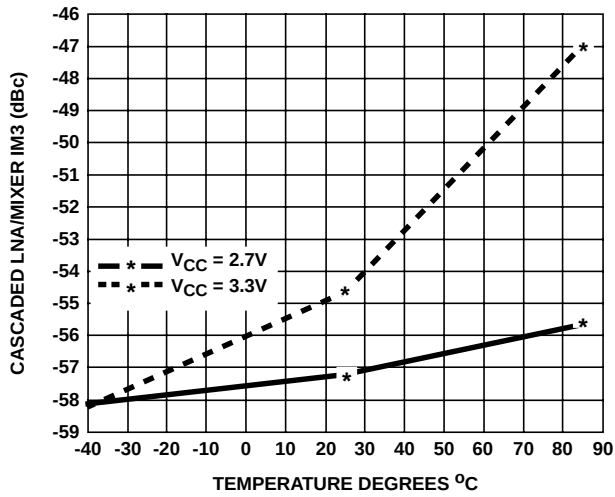
FIGURE 32. RX OUTPUT IM3 AT -12dBm INPUT TONES
