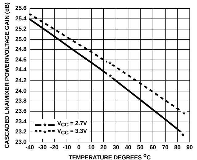
FIGURE 27. POWER/VOLTAGE GAIN HIGH GAIN MODE
