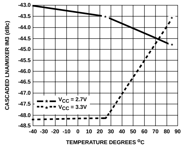
FIGURE 31. RX OUTPUT IM3 AT -5dBm INPUT TONES
