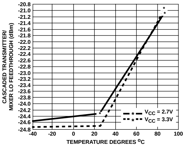
FIGURE 42. LO TO TRANSMIT AMP OUTPUT FEEDTHROUGH (CASCADED, NO FILTER)
