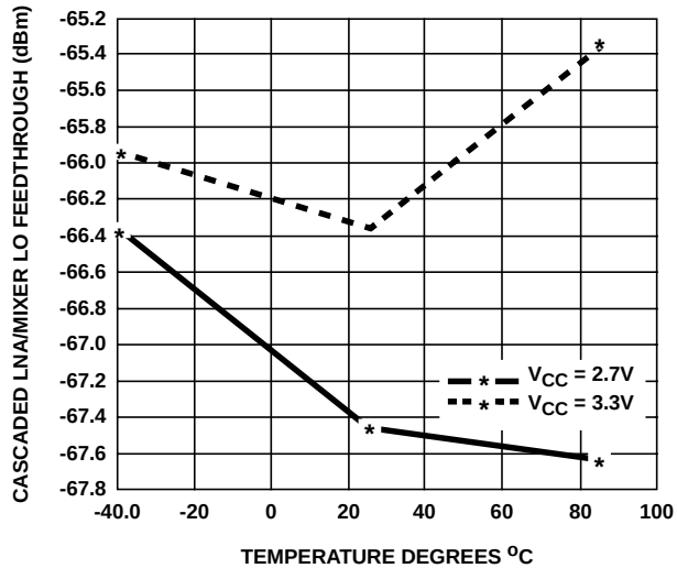
FIGURE 38. LO TO LNA INPUT FEEDTHROUGH (CASCADED, NO FILTER)
