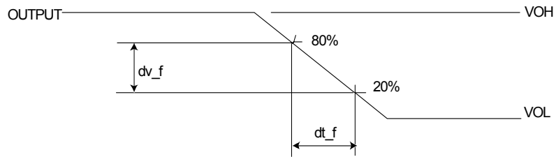
Figure 20. High to Low Slew Rate Measurement
