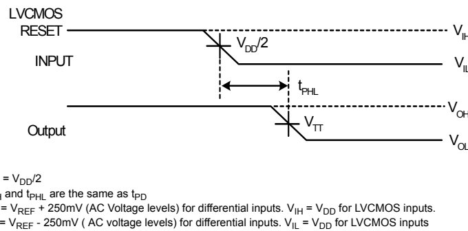
Figure 29. Partial-parity-out ; propagation delay times with respect to clock inputs
