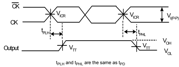
Figure 17. Propagation Delay
