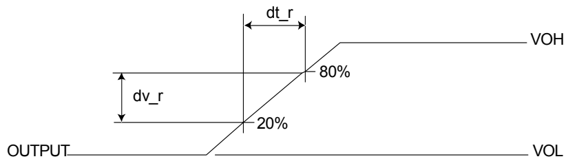
Figure 22. Low to High Slew Rate Measurement
