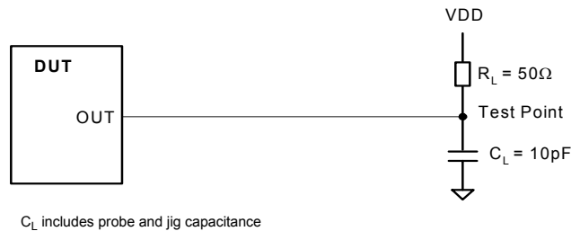
Figure 19. Load Circuit - High to Low Slew Measurement
