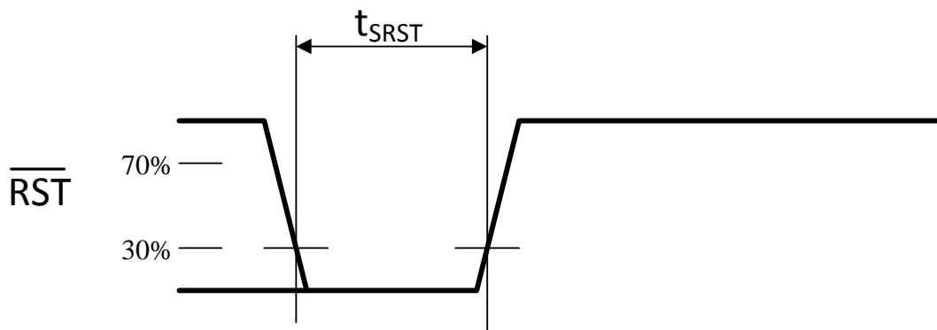
Figure 1. Reset Timing
