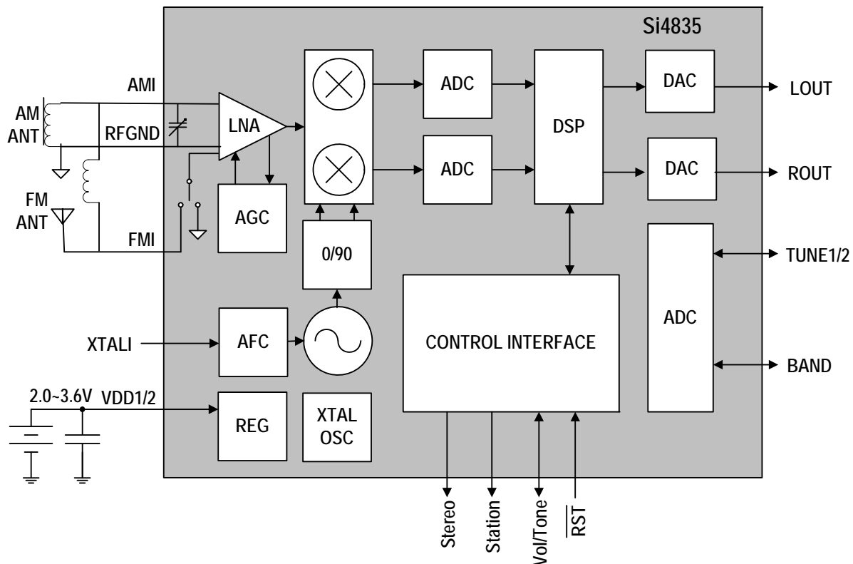
Figure 2. Si4835-B31 Functional Block Diagram
