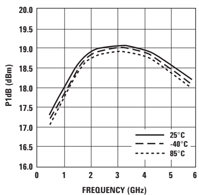
Figure 18. P1dB vs. Frequency and Temp. Tuned for Max OIP3 and Fmin at 3V, 30 mA.
