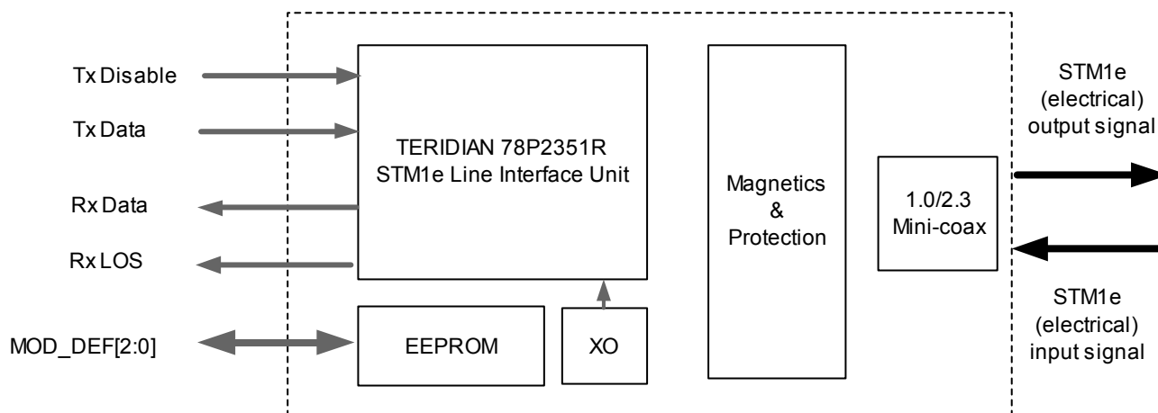
Figure 1: Transceiver Functional Diagram
