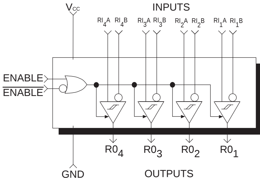
Figure 1. SP26LV432 Block Diagram
