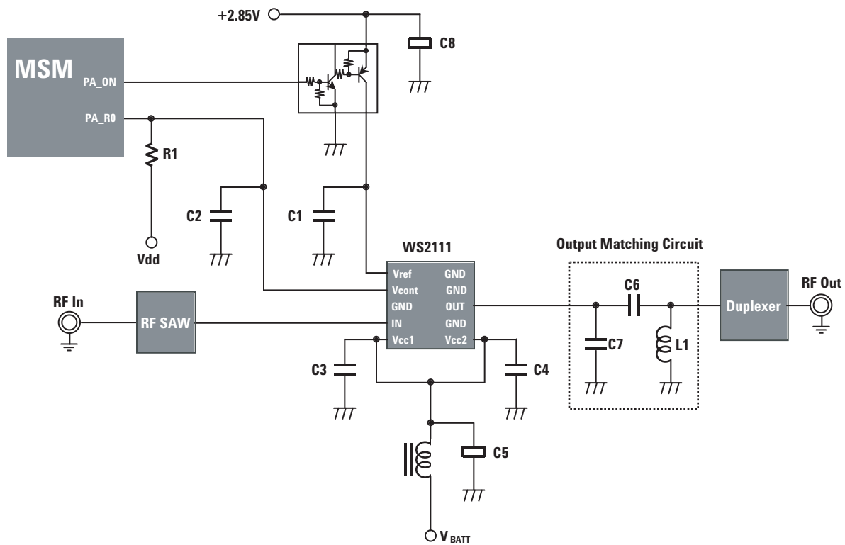
Figure 21. Peripheral Circuit.
