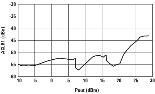
Figure 9. Adjacent Channel Leakage Ratio 1 vs. Output Power.
