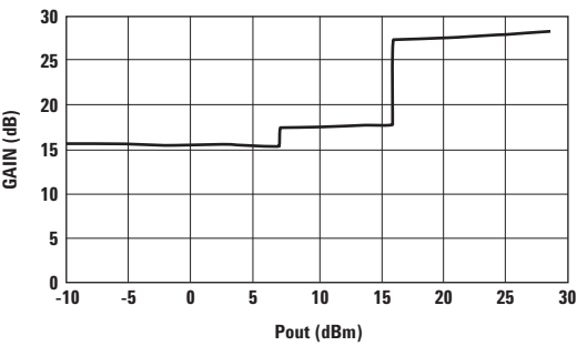
Figure 7. Gain vs. Output Power.
