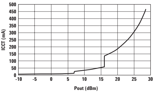
Figure 6. Total Current vs. Output Power.
