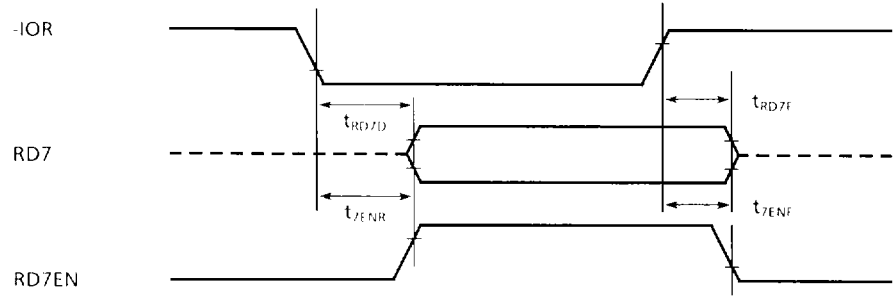
7) Wave form of RD7, RD7EN
