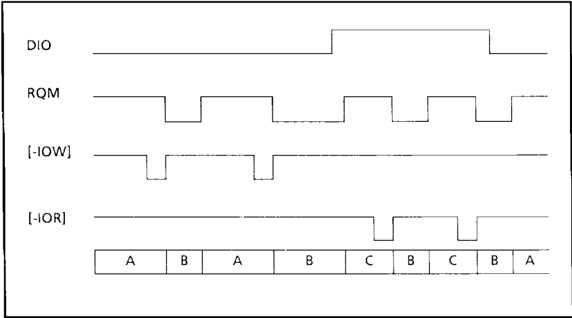
FIG.5.2.2 MAIN STATUS REGISTER TIMING
