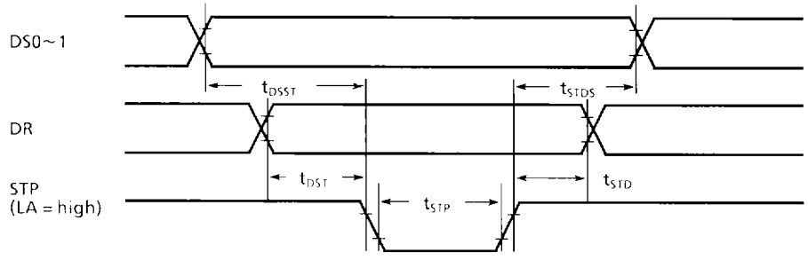
6) Seek Operation ( For CDS = Low, DS0~1 )
