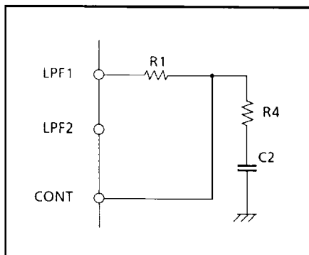
FIG.5.3.4b FILTER CIRCUIT
