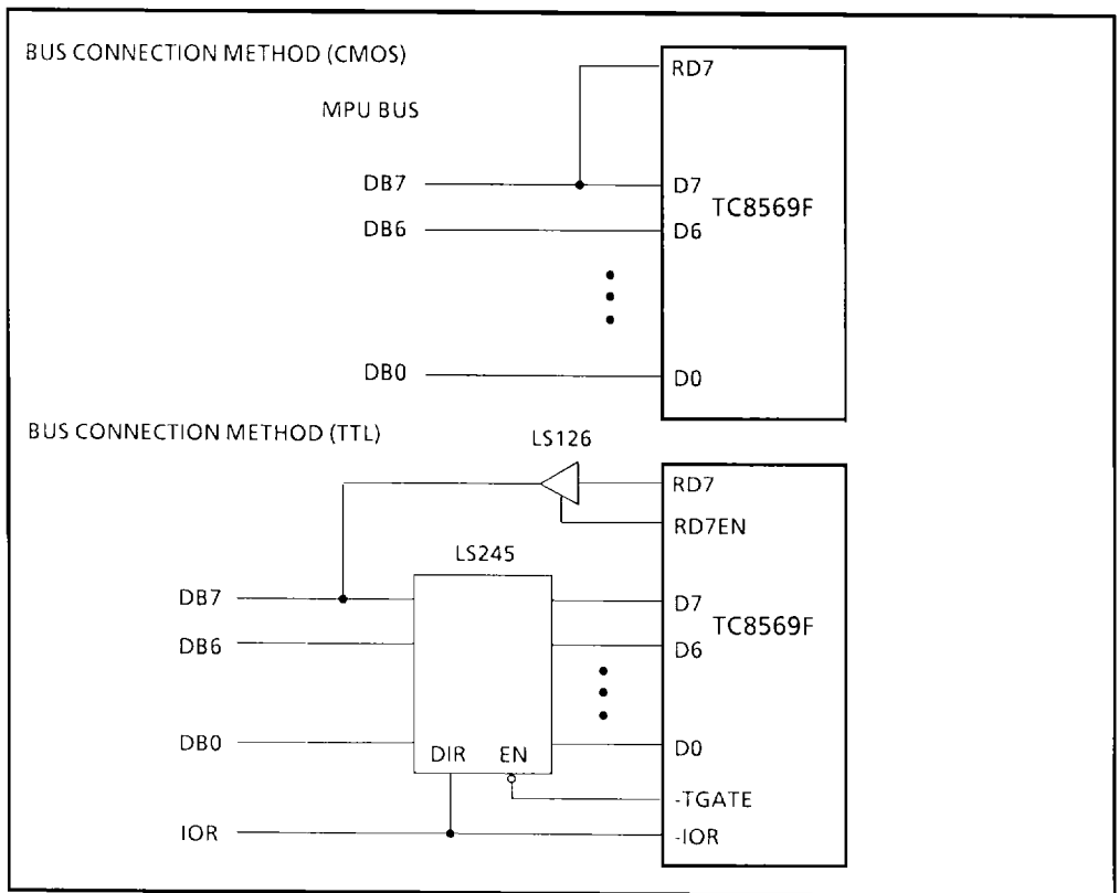
FIG. 5.1.5 BUS CONNECTION METHOD
