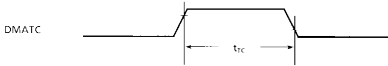
5) Wave form of Terminal Count
