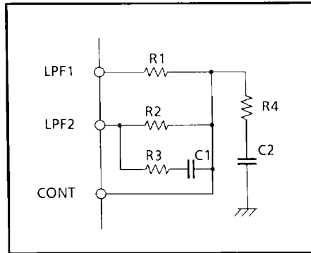
FIG. 5.3.4 FILTER CIRCUIT
