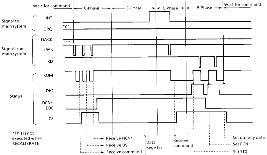
FIG 5.3e SEEK, RECALIBRATE & FIG 5.3f SENSE INTERRUPT STATUS
