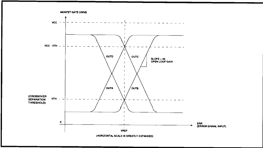
FIGURE 5: Crossover Protection
