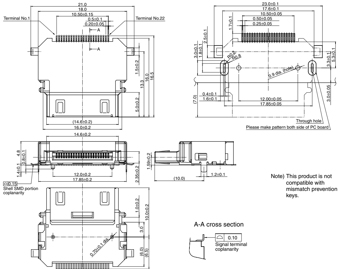
Recommended PC board pattern (TOP VIEW)
