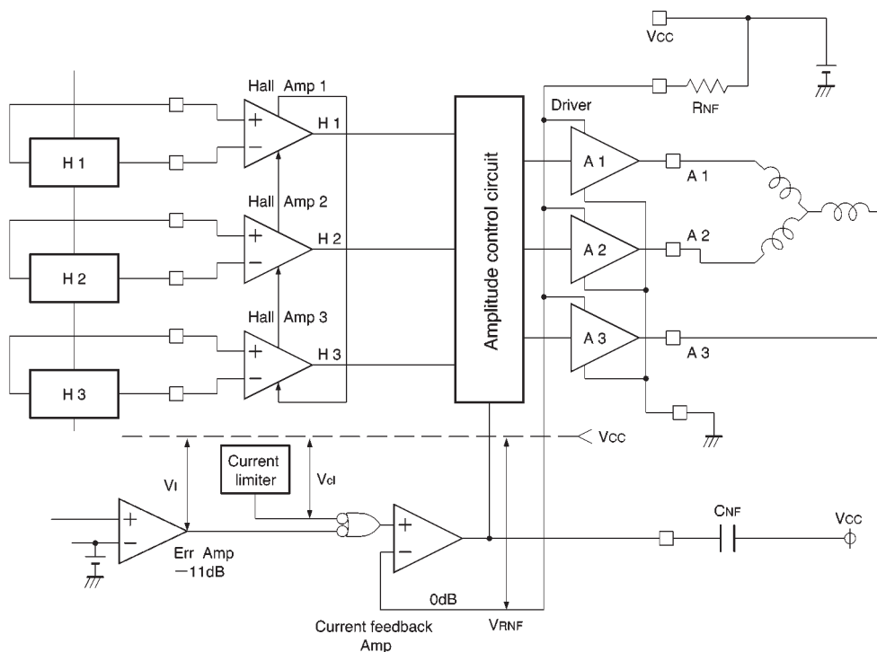
Fig.1 Motor drive circuit
