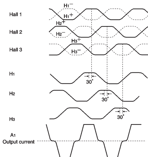
Fig.2 I/O waveforms
