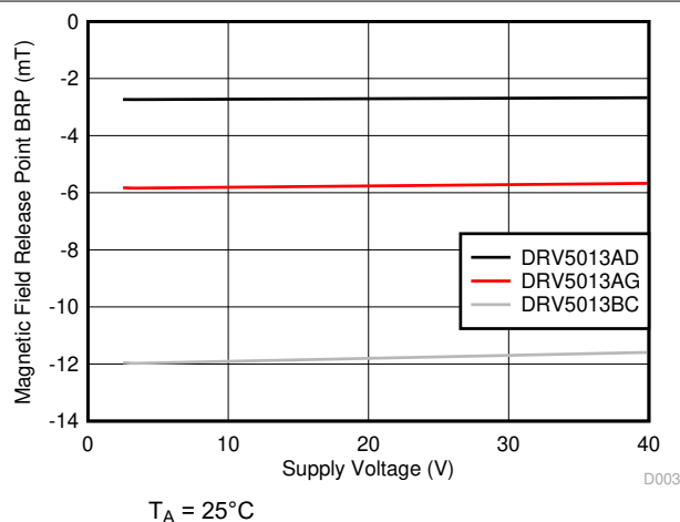
Figure 6-5. B_{RP} vs V_{CC}
