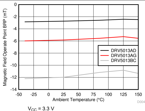
Figure 6-6. B_{RP} vs Temperature
