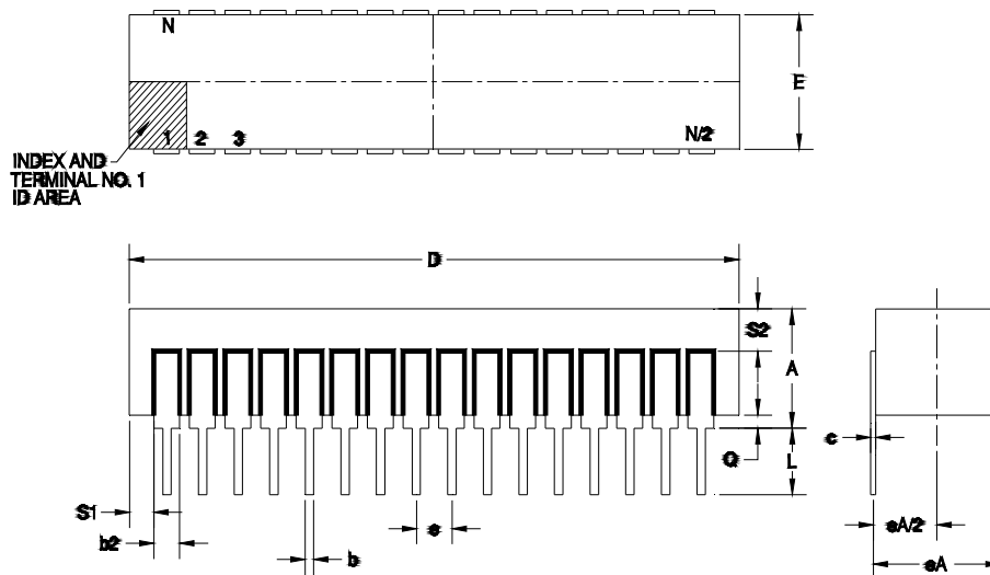
32 PIN DUAL IN-LINE PACKAGE 1,2
