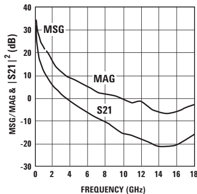
Figure 38. MSG/MAG & |S_{21}|^2 vs Frequency at 3.5V/200 mA.
