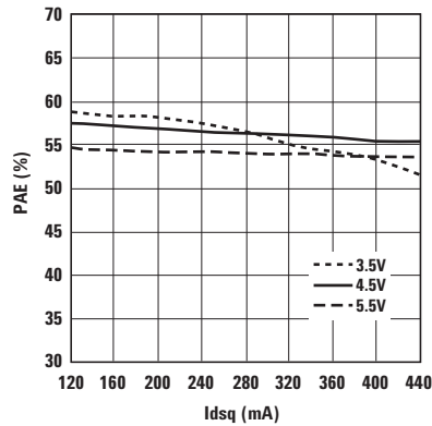
Figure 26. PAE vs. I_{dsq} and V_d at 900 MHz.
