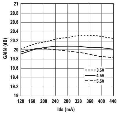
Figure 25. Gain vs. I_{ds} and V_d at 900 MHz.
