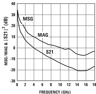
Figure 32. MSG/MAG & |S_{21}|^2 vs Frequency at 4.5V/200 mA.
