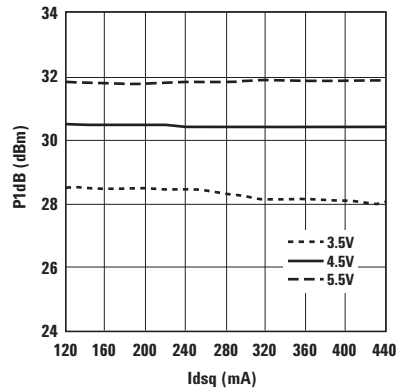
Figure 24. P1dB vs. I_{dsq} and V_d at 900 MHz.
