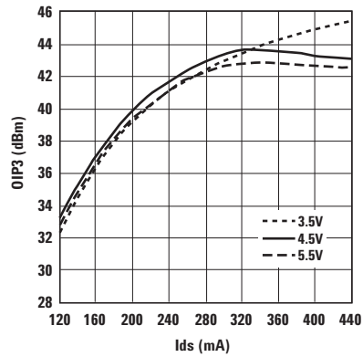
Figure 23. OIP3 vs. I_{ds} and V_d at 900 MHz.
