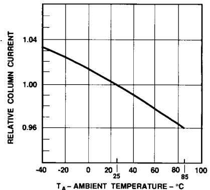
Figure 4. Relative Column Current, I_{\text{COL}} , vs. Ambient Temperature.
