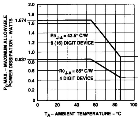
Figure 1. Maximum Allowable Power Dissipation vs. Ambient Temperature as a Function of Thermal Resistance IC Junction-to-Ambient, R_{\theta_{J-A}} . Operation at 85^\circ\text{C} Assumes a Thermal Resistance for the Printed Circuit Board of R_{\theta_{PC-A}} = 35^\circ\text{C/W} Per Device for the HCMS-270X, 17.5^\circ\text{C/W} Per Device for the HCMS-271X, and 17.5^\circ\text{C/W} Per Row for the HCMS-272X.
