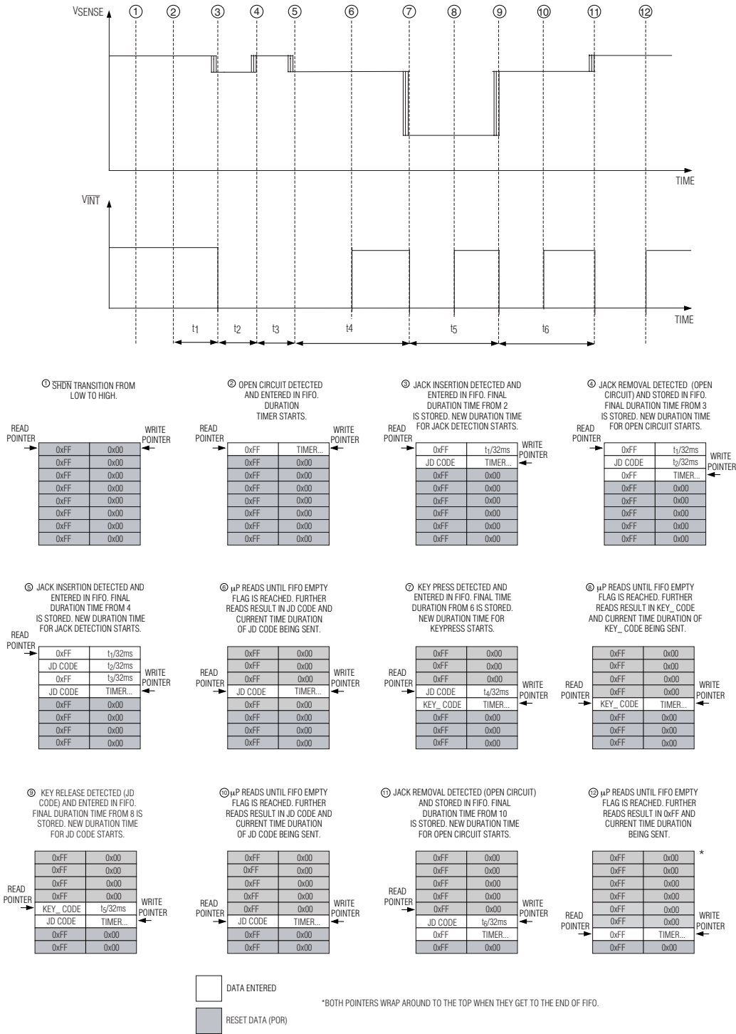
Figure 10. Power-Up, Jack Detect, and Keypress Example
