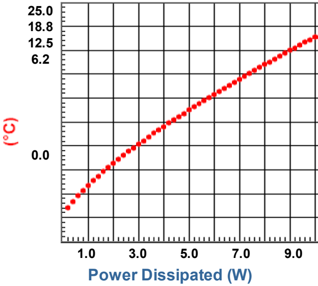
Heat Sink Temperature Rise Above Ambient
