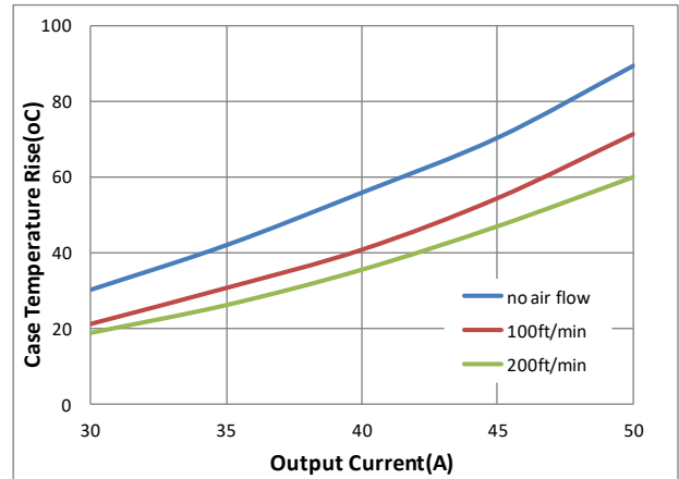
Figure 9: IOUT_MAX Derating Curve
