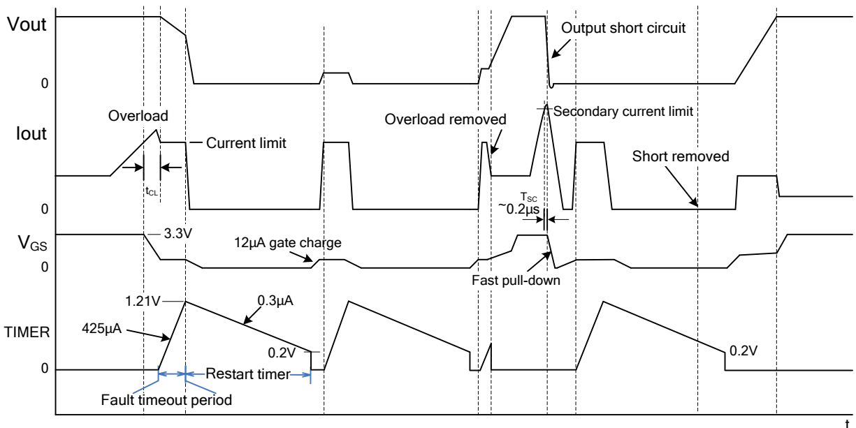
Figure 3: Over-Current Protection (Auto-Retry Mode, F0h AUTO bit = 1)
