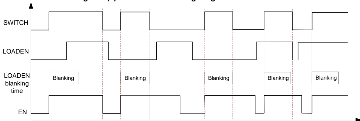
Figure 7(b): EN/LOADEN Timing Diagram at Auto-Retry mode
