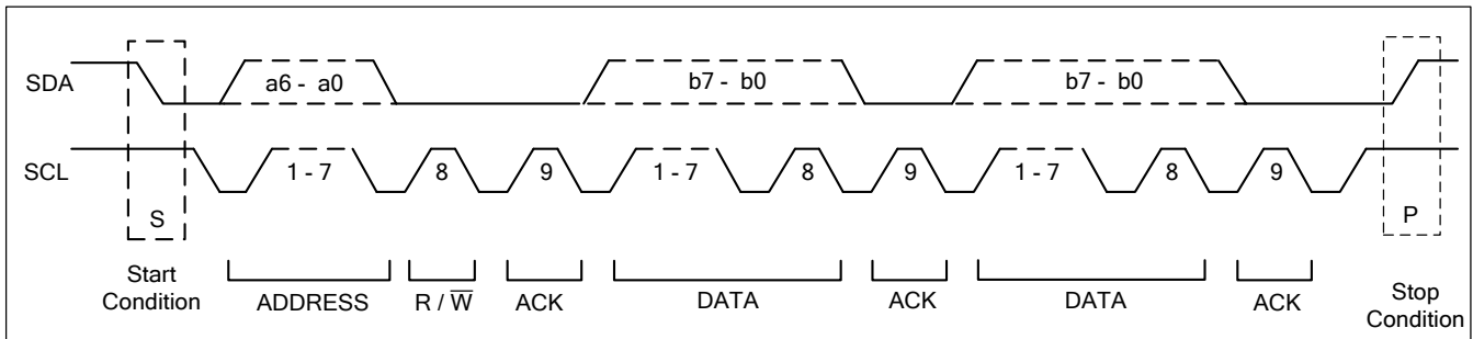
Figure 14: Data Transfer over PMBus™
