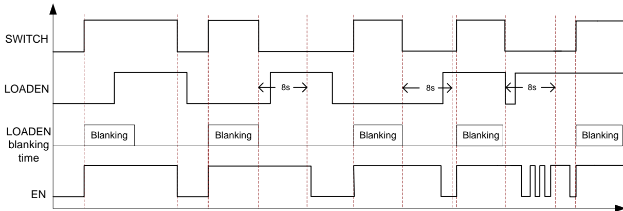
Figure 7(a): EN/LOADEN Timing Diagram at Latch-Off mode
