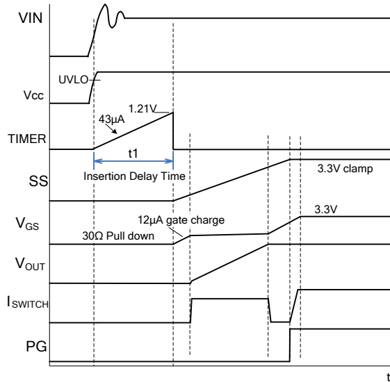
Figure 5: Start-Up Sequence
