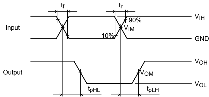
Figure 2 t_{pLH} , t_{pHL}
