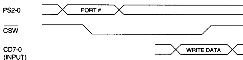
CPU-PVDC WRITE CYCLE
