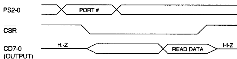
CPU-PVDC READ CYCLE
