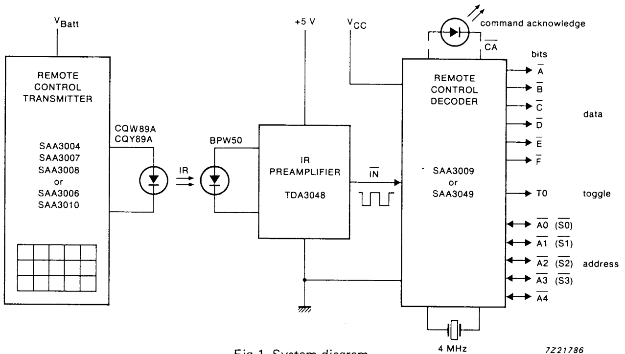
Fig.1 System diagram.
