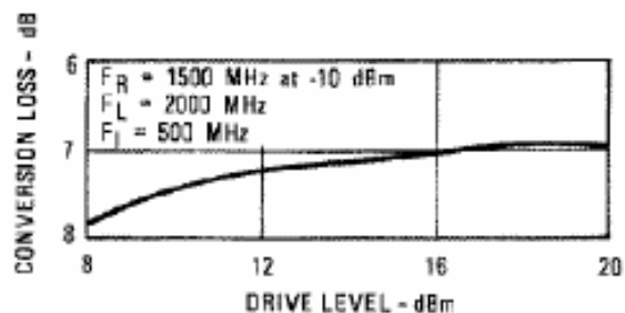
Conversion Loss
