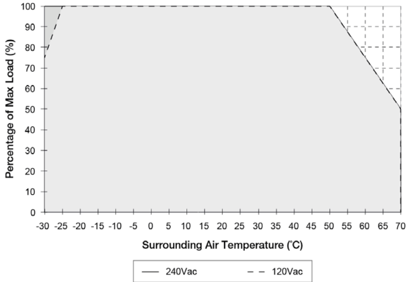
Fig. 1 De-rating for Vertical and Horizontal Mounting Orientation 120Vac < -25°C de-rate power by 5.0% / °C 120Vac and 240Vac > 50°C de-rate power by 2.5% / °C
