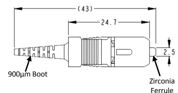
SC Simplex Connector with 900µm Boot
