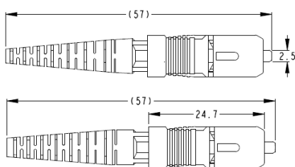
SC Simplex Connector with 2.0mm and 3.0mm Boots
