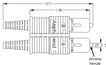
SC Duplex Connector with 3.0mm Boots
