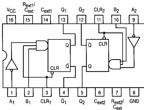
LOGIC DIAGRAM
