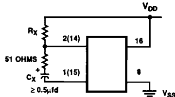
FIGURE 2. ALTERNATE RAPID POWER-DOWN PROTECTION CIRCUIT
