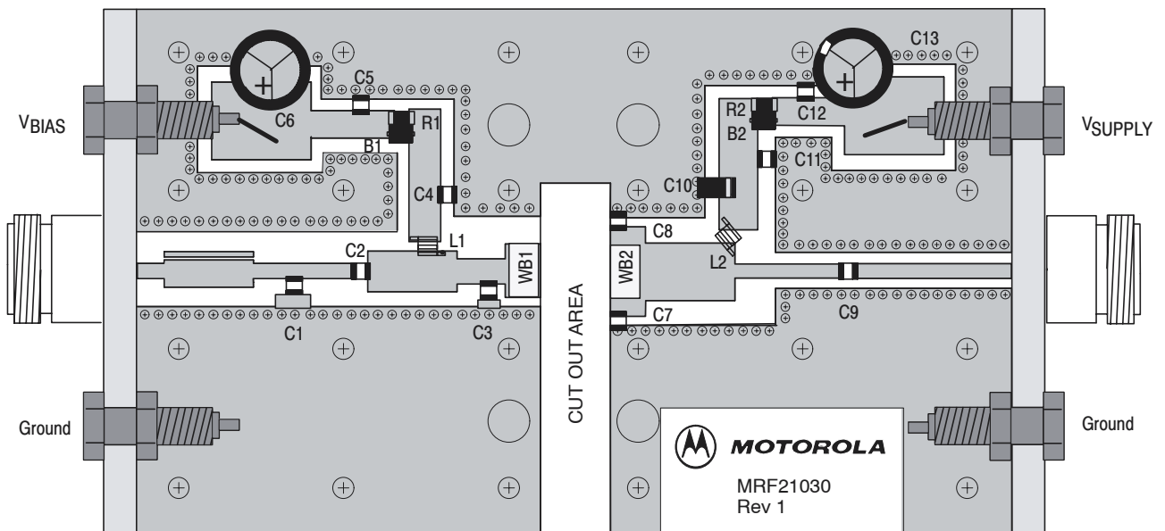
Figure 2. MRF21030 Test Circuit Component Layout
