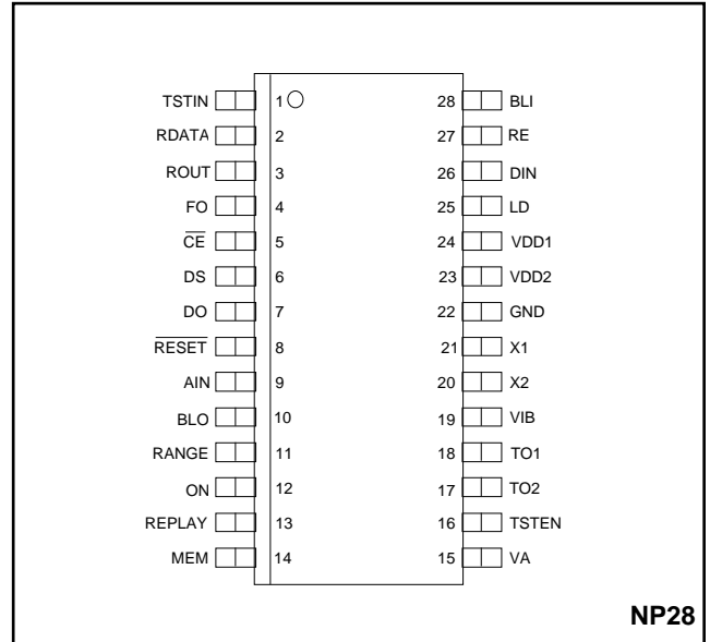
Fig. 1 Pin connection (top view - not to scale)
