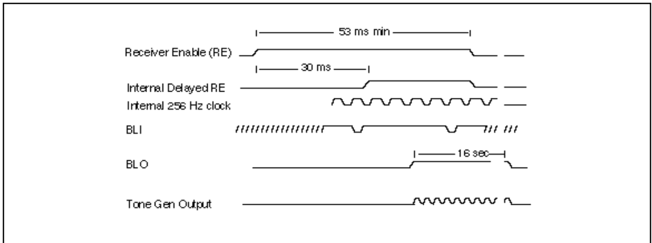
Fig. 8 Battery Low Detect Circuit Timing
