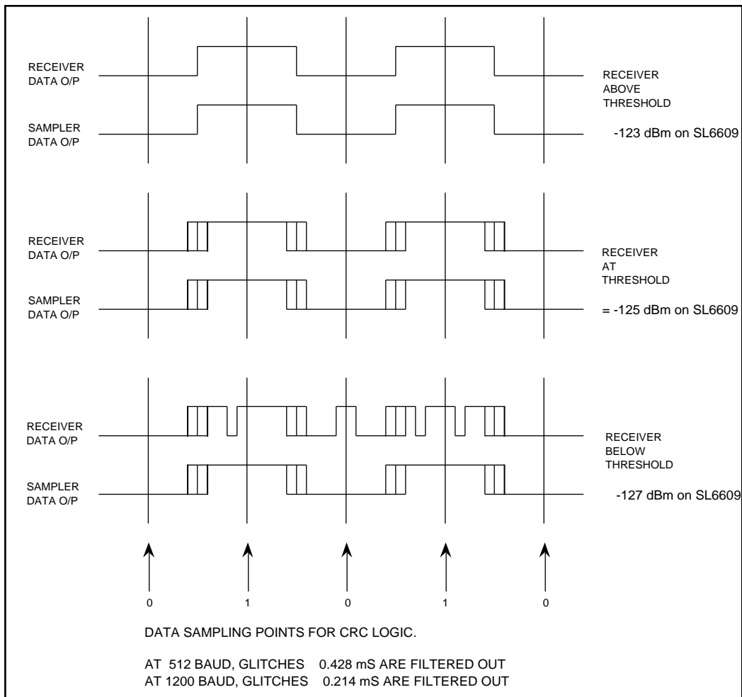
Fig. 4 Data Filter Operation
