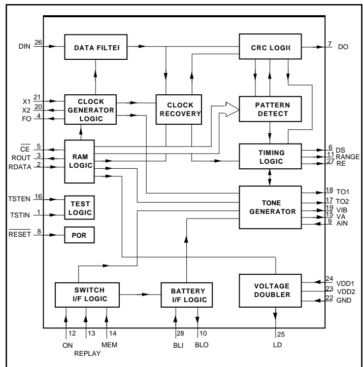
Fig. 2 MV6639 Block Diagram
