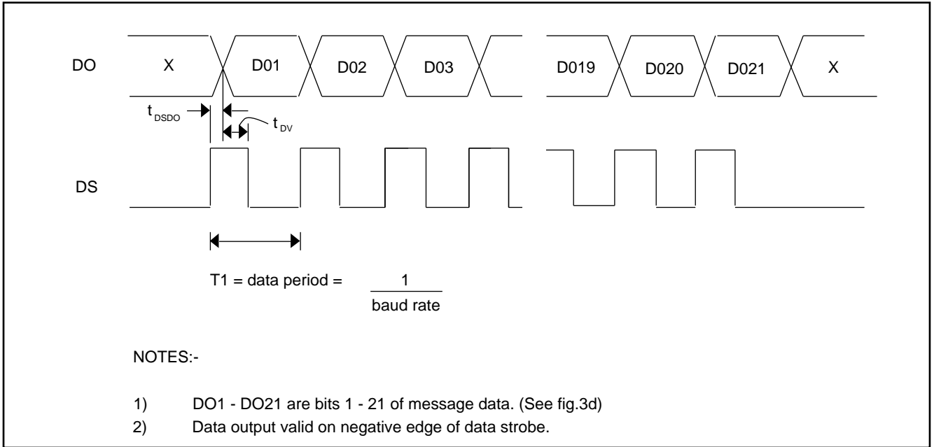
Fig. 5 Data Output Timing
