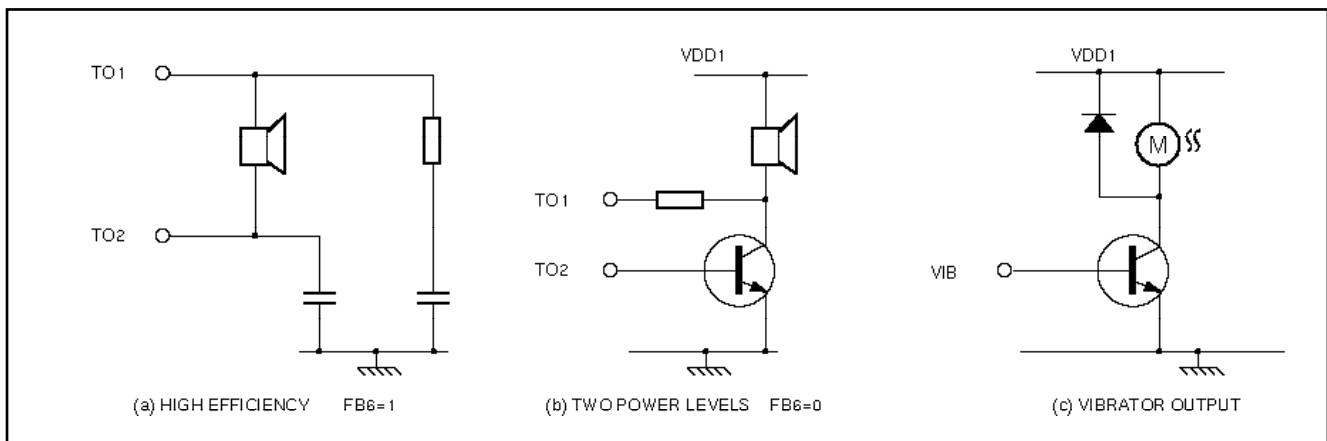
Fig. 10 Tone Generator / Vibrator Interface Circuits
