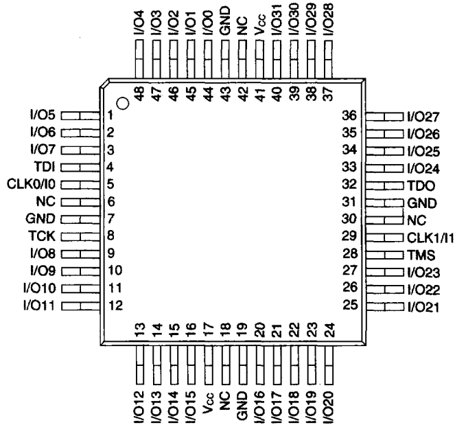
48-Pin TQFP
