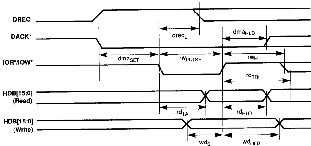
Figure 9-12. Host DMA 8-/16-Bit Interface Timing (Demand Mode)
