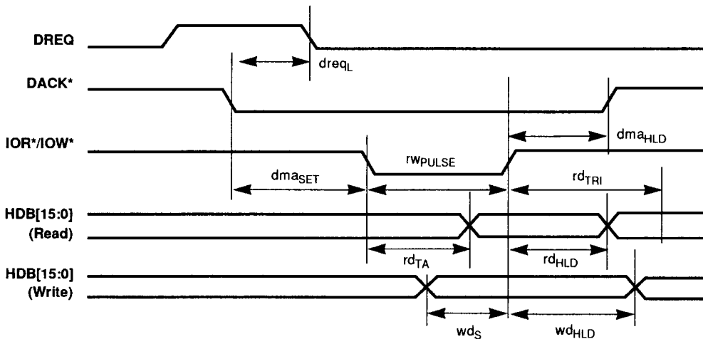
Figure 9-11. Host DMA 8-/16-Bit Interface Timing (Single-Transfer Mode)
