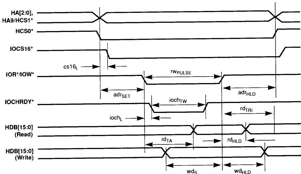
Figure 9-10. Programmed I/O, 8-/16-Bit Host Interface Timing
