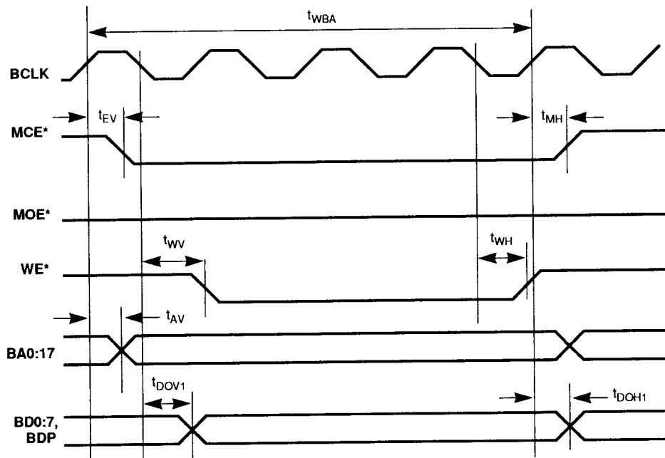
Figure 9-8b. SRAM Write Timing
