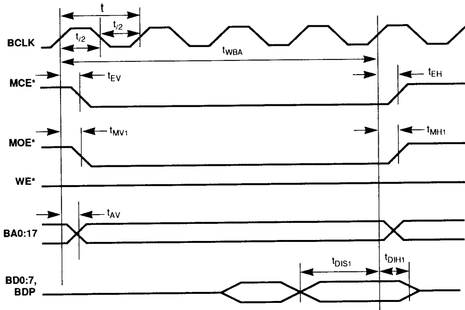
Figure 9-8a. SRAM Read Timing
