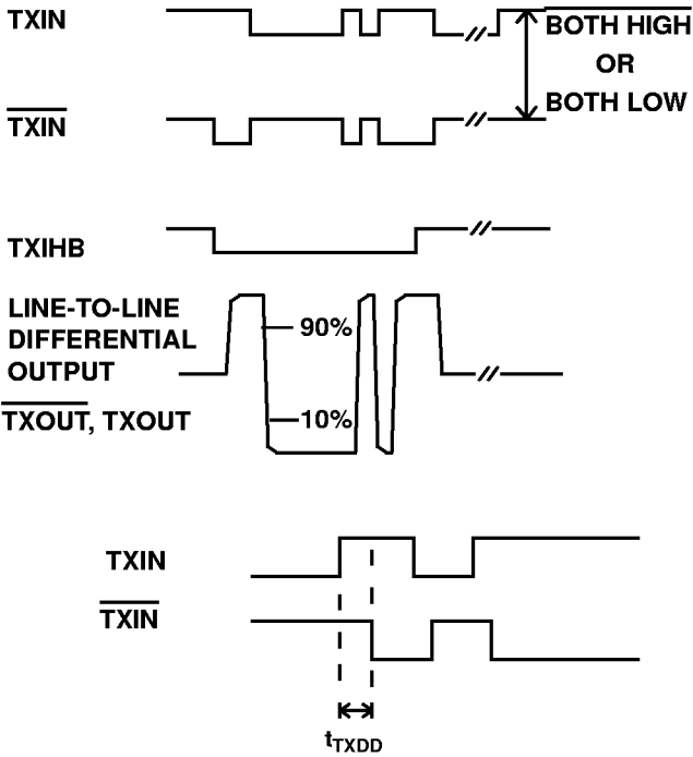
Figure 3. Typical Transmitter Waveforms
