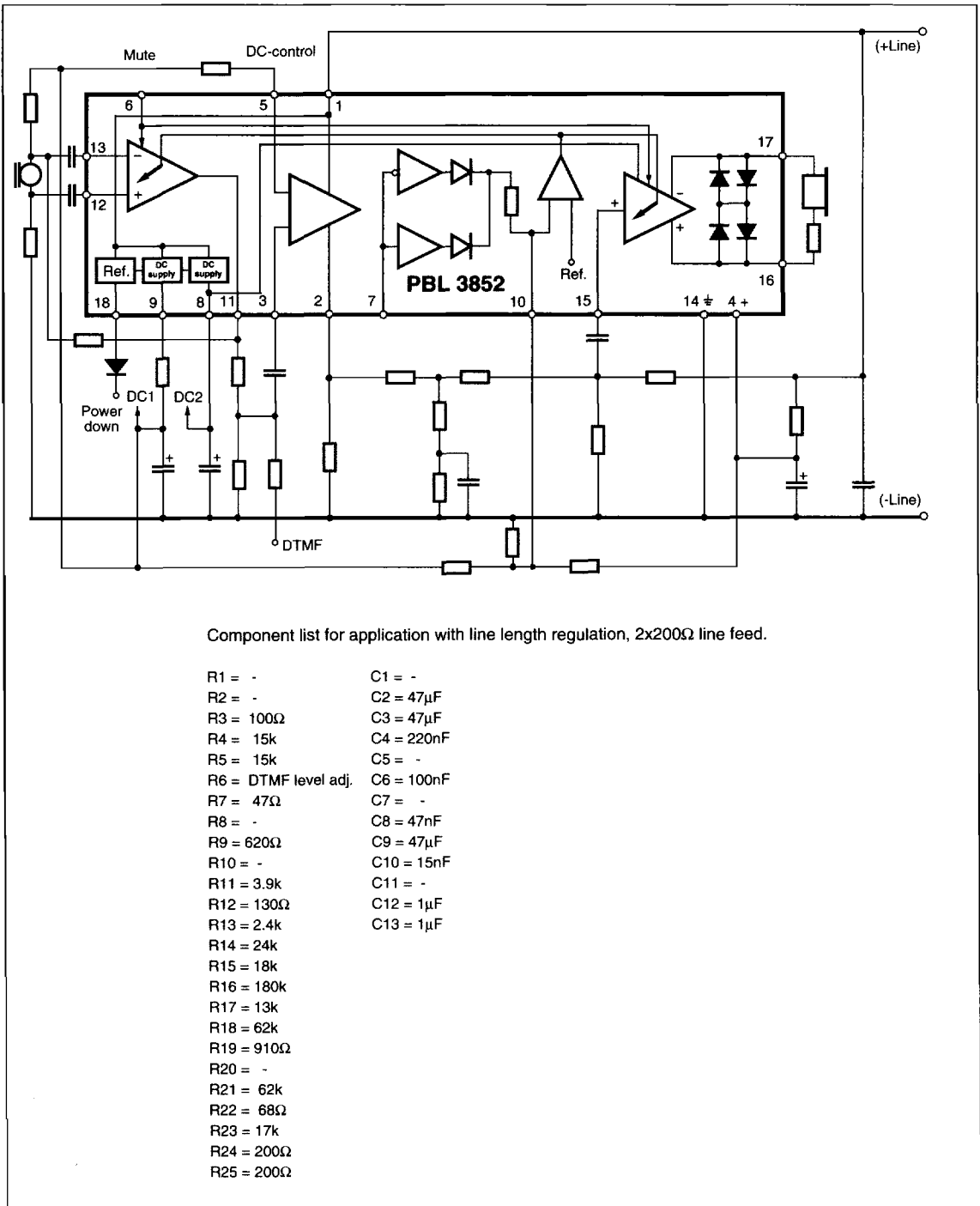
Figure 33. Application with line length regulation, 2x200Ω line feed.
