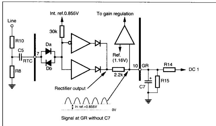
Figure 18. The dynamic limiter function
