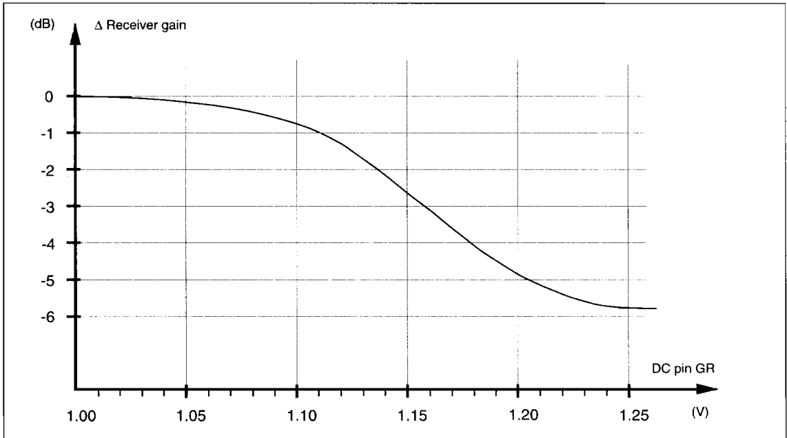
Figure 16. Receiver line length regulation.
