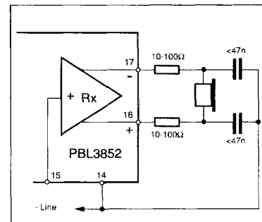
Figure 28. RFI elimination at receiver amplifier output.
