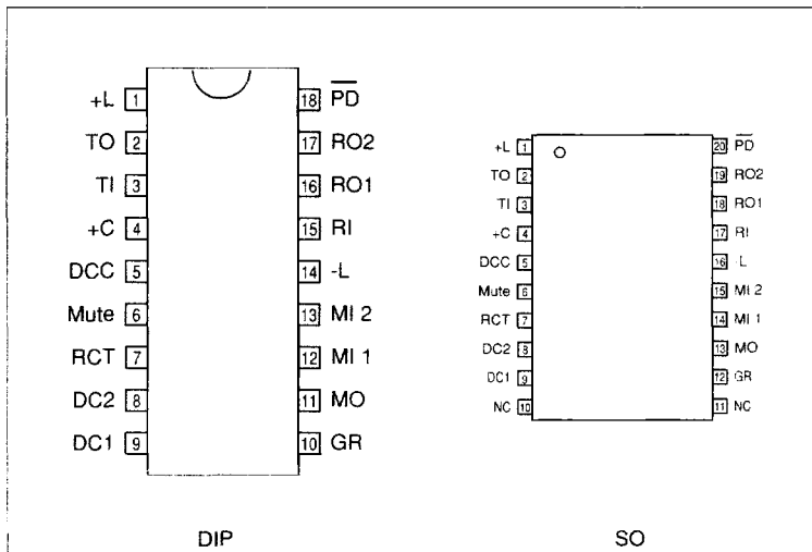
Figure 5. Pin configuration.
