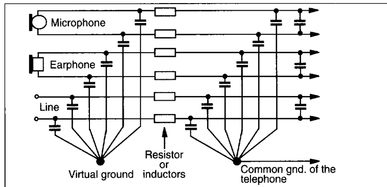
Figure 31. RFI elimination in the wiring.
