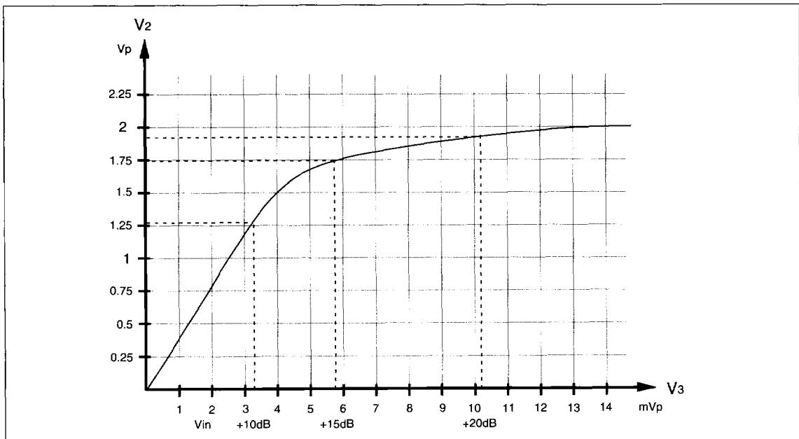
Figure 17. Dynamic limiter.
