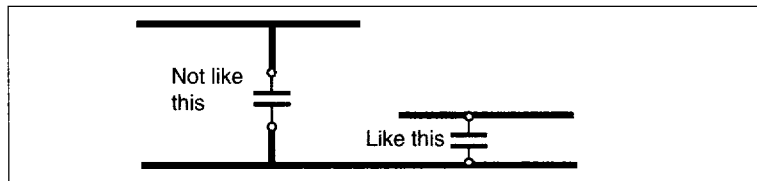
Figure 30. RFI elimination at PCB layout level.
