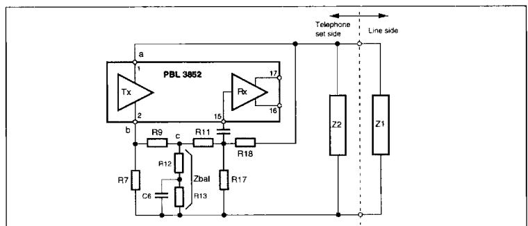
Figure 26. The side tone suppression principle.
