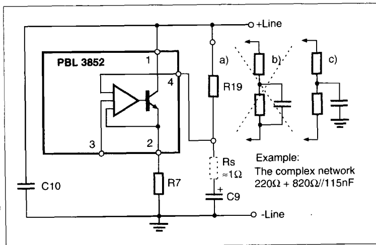
Figure 6. AC-impedance.
