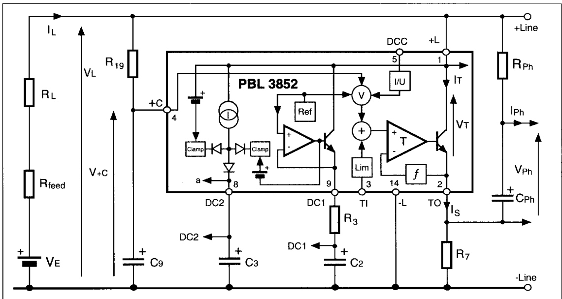
Figure 22. DC-supplies.
