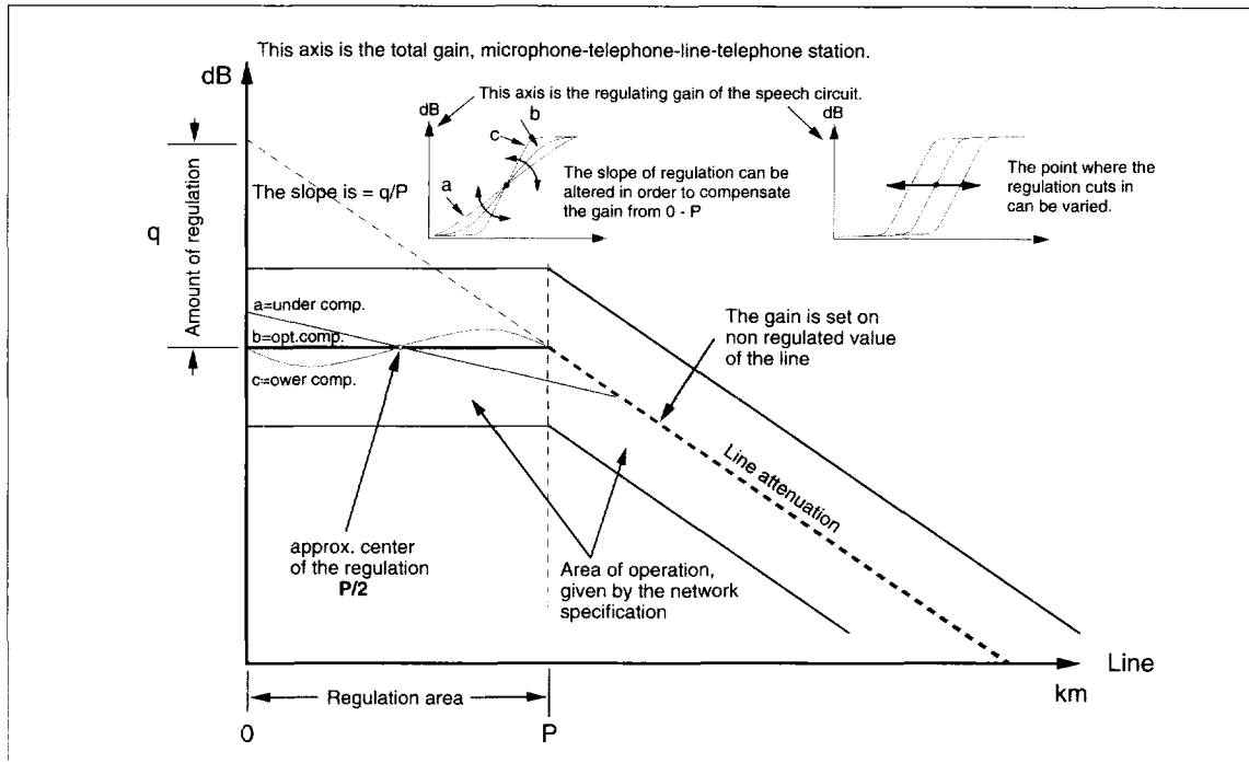
Figure 13. Line length regulation.
