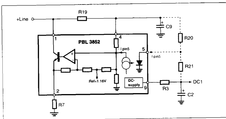
Figure 7. System of DC-Characteristic.
