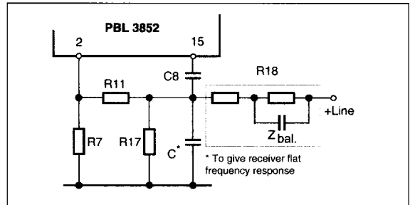
Figure 25. Side tone network with complex R18.
