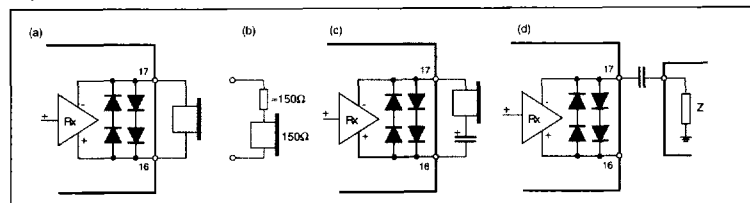
Figure 12. Receiver arrangements.
