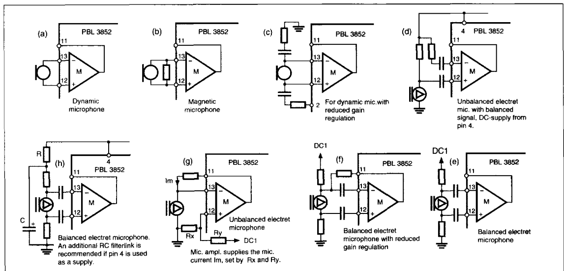
Figure 10. Microphone solutions.
