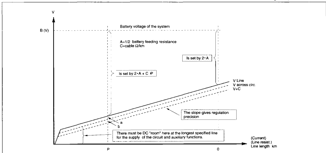
Figure 14. The DC-characteristic of a telephone.
