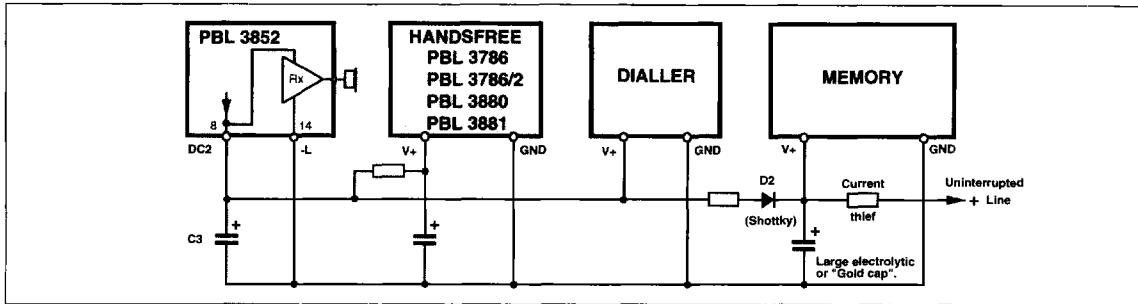
Figure 23. DC-2 supply of peripheral circuits and memory retention.
