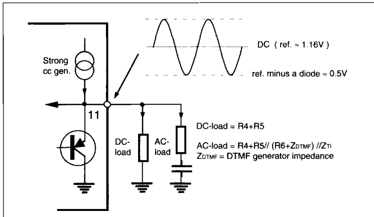
Figure 9. Microphone amplifier output clipping.
