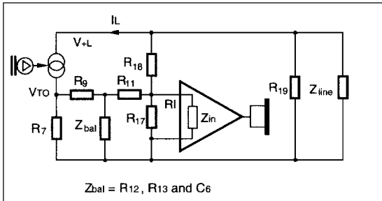
Figure 24. Sidetone balance.
