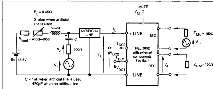
Figure 2. Test set up without rectifier bridge.
