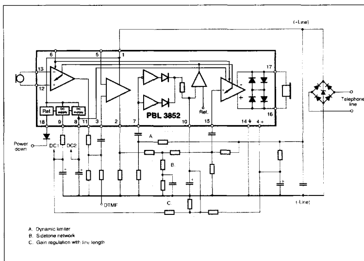
Figure 1. Functional diagram.
