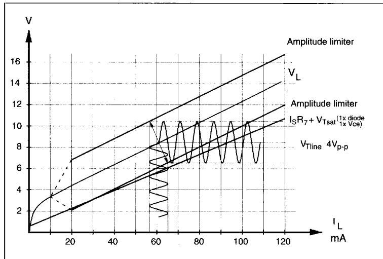
Figure 19. Transmitter output signal limiter. See fig. 22 for data.
