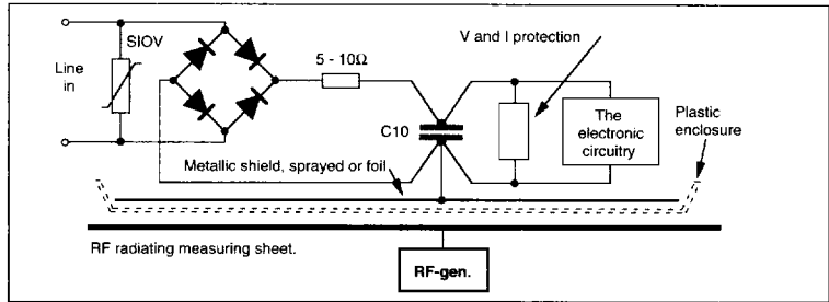
Figure 29. Measuring RFI.
