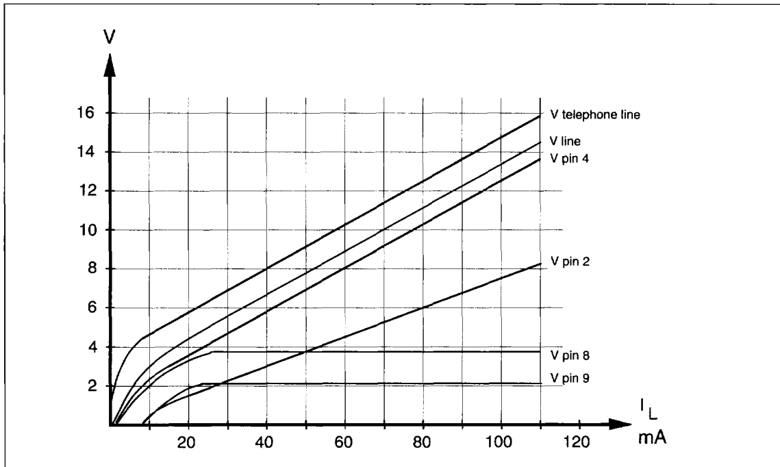
Figure 8. DC-Characteristics. ( R_7 = 75 \Omega )
