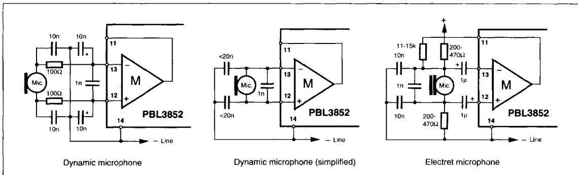
Figure 27. RFI elimination at microphone amplifier input .
